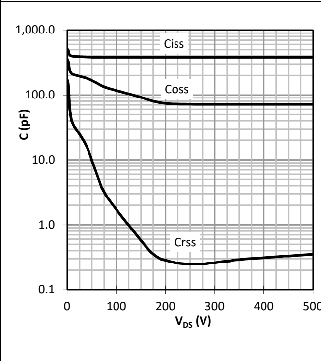
Figure 20 Typ. capacitances
