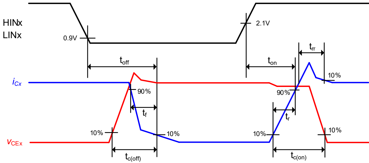
Figure 9 Switching times definition of inverter part
