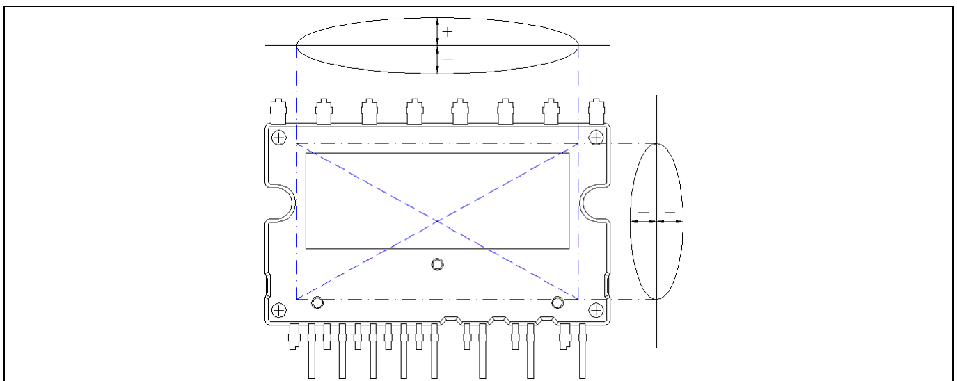
Figure 8 Backside curvature measurement position
