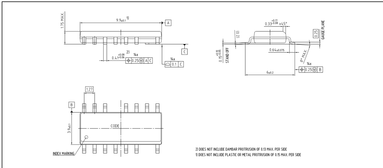
Figure 15 PG-DSO-14
