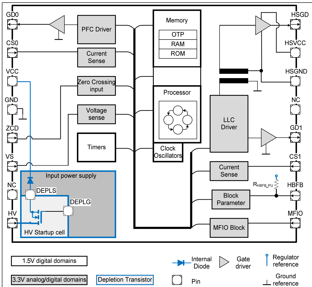
Figure 3 Representative Blockdiagram
