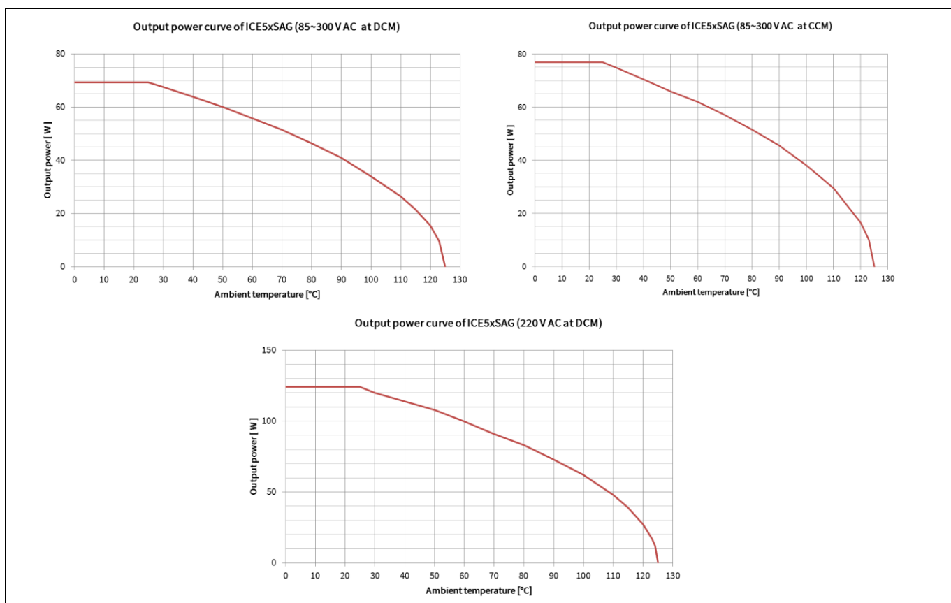
Figure 17 Output power curve of ICE5xSAG
