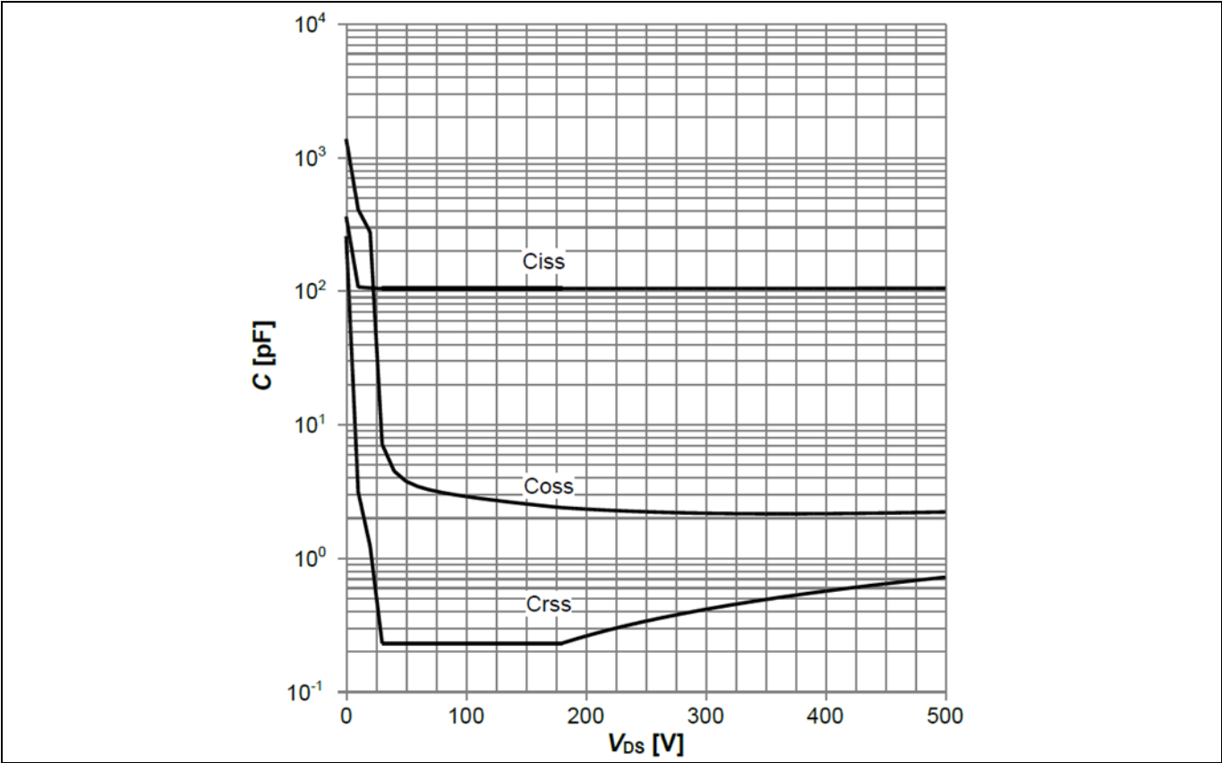
Figure 23 Typical CoolMOS™ capacitances of ICE5QR4780BG ( C=f(V_{DS}) ; V_{GS}=0 V; f=250 kHz)
