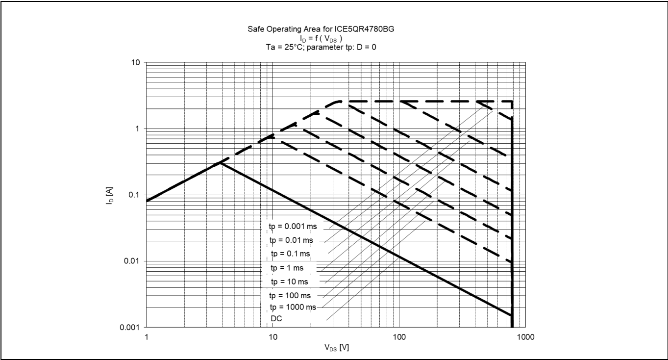
Figure 14 Safe Operating Area (SOA) curve for ICE5QR4780BG
