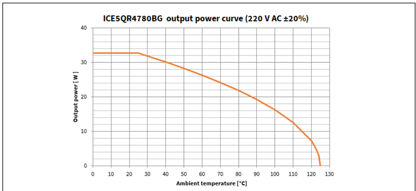
Figure 28 Output power curve of ICE5QR4780BG, V_{IN}=220\text{ V}_{AC} ; P_{Out}=f(T_a)
