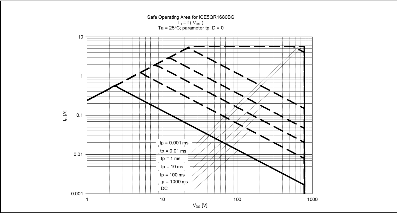
Figure 16 Safe Operating Area (SOA) curve for ICE5QR1680BG
