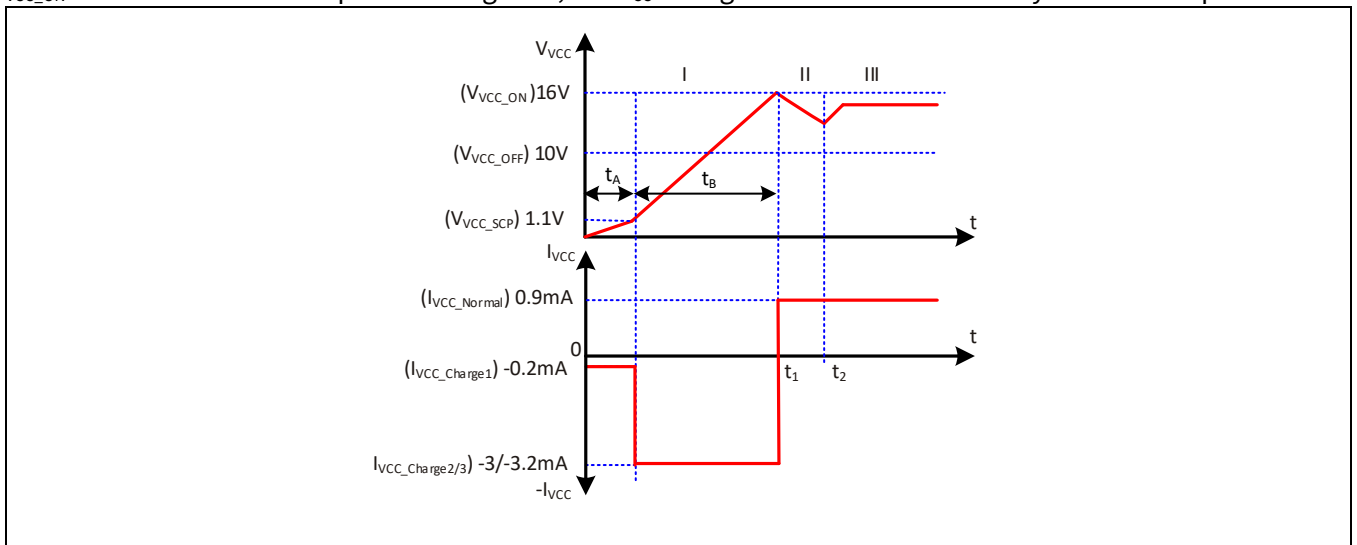
Figure 4 VCC voltage and current at start up
