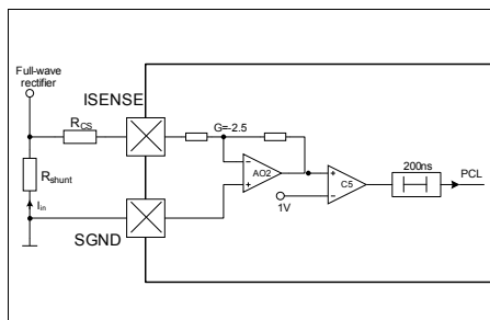
Figure 12 Peak Current Limit (PCL)
