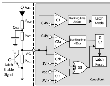
Figure 32 Latch and fast AC reset
