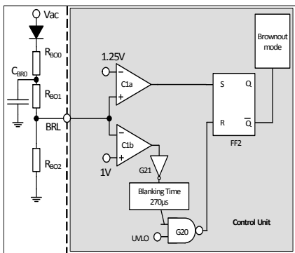
Figure 30 Brownout detection circuit
