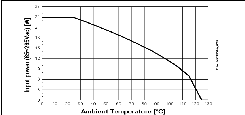
Figure 38 Input power curve V_{in}=85-265V_{ac} ; P_{in}=f(T_a)
