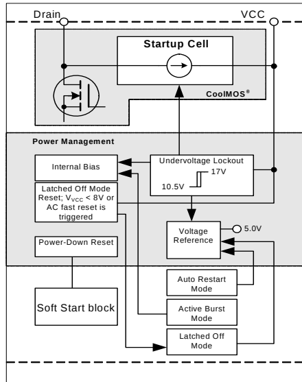
Figure 3 Power Management
