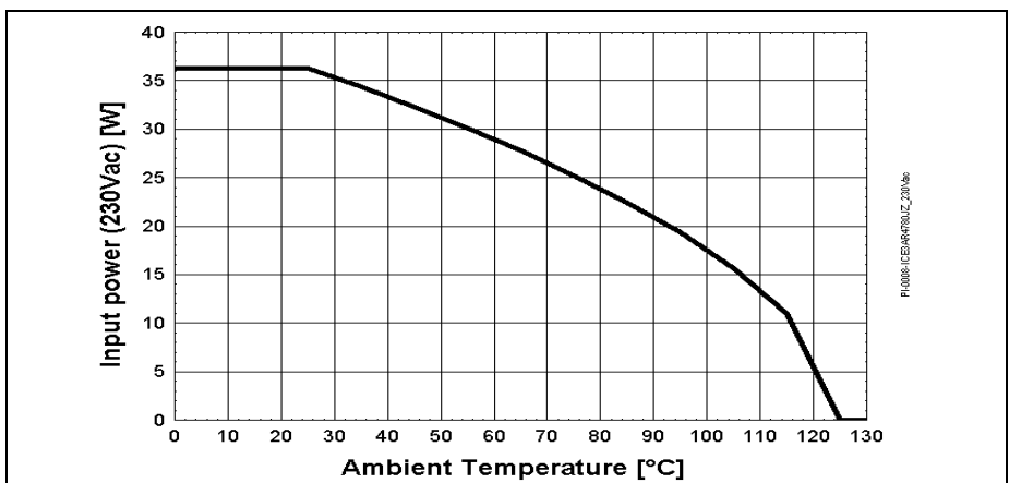
Figure 39 Input power curve V_{in}=230V_{ac}+/-15\% ; P_{in}=f(T_a)
