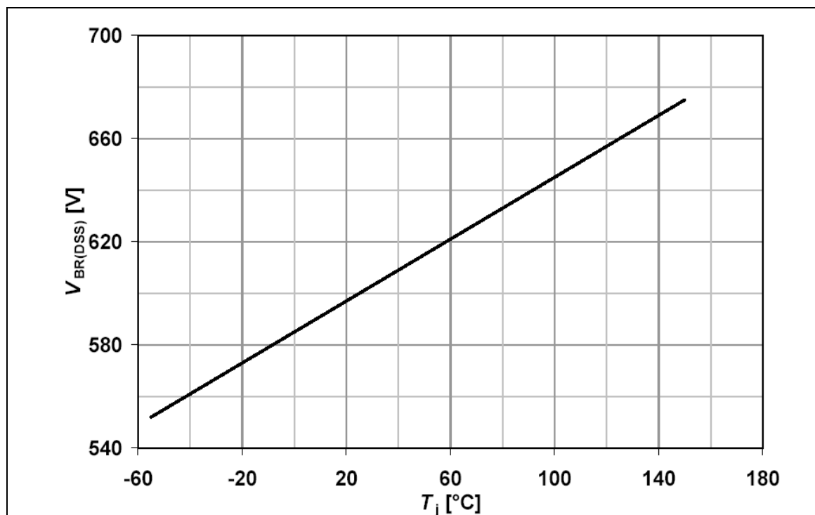
Figure 11 Drain-source breakdown voltage; V_{BR(DSS)}=f(T_j)
