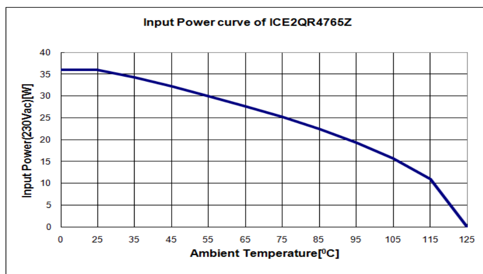
Figure 13 Input Power curve V_{in}=230V_{ac}; P_{in}=f(T_a)
