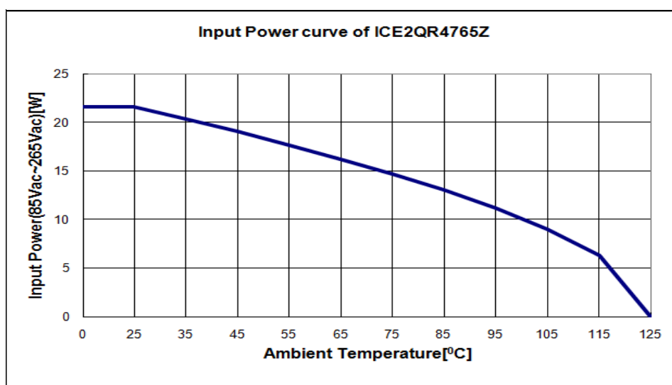
Figure 12 Input Power curve V_{in}=85\sim 265V_{ac}; P_{in}=f(T_a)
