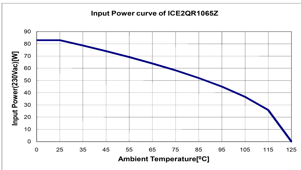
Figure 13 Input Power curve V_{in}=230V_{ac} ; P_{in}=f(T_a)
