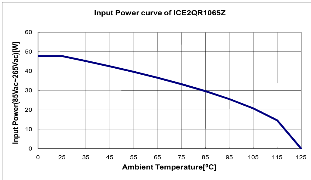
Figure 12 Input Power curve V_{in}=85\sim 265V_{ac} ; P_{in}=f(T_a)
