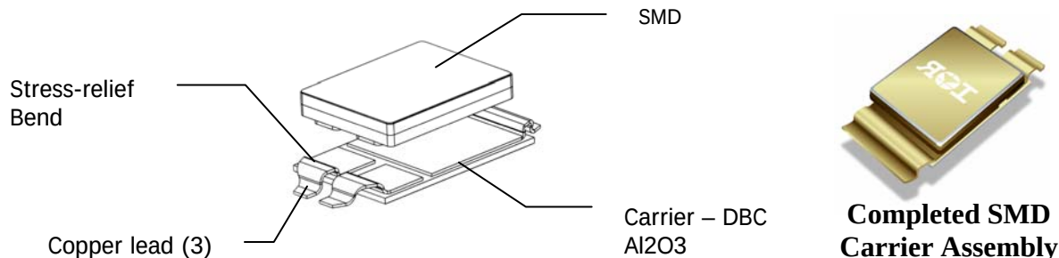
Figure 11. SMD Carrier Assembly
