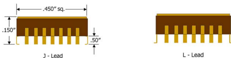
Figure 8. CLCC Gull-Wing Leads Attachment
