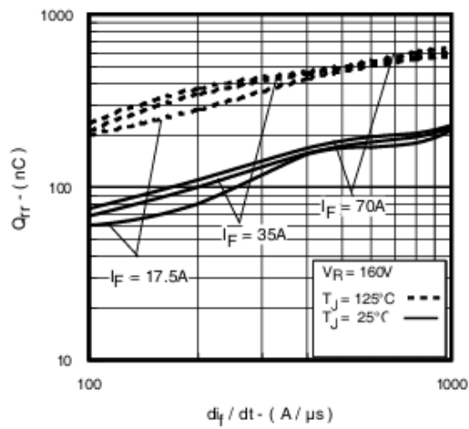
Figure 7 Typical Stored Charge Vs. di_f/dt
