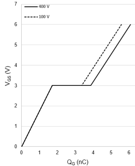
Gate Charge, Q_G Characteristic
