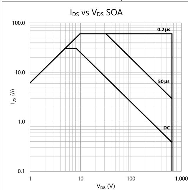
Figure 13: Safe Operating Area @ T_{case} = 25^{\circ}\text{C}
