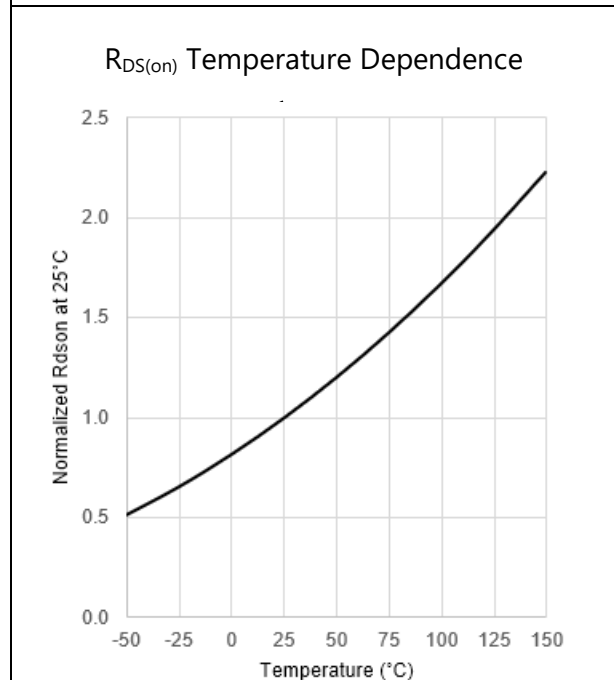
Figure 12: Normalized R_{DS(on)} as a function of T_J
