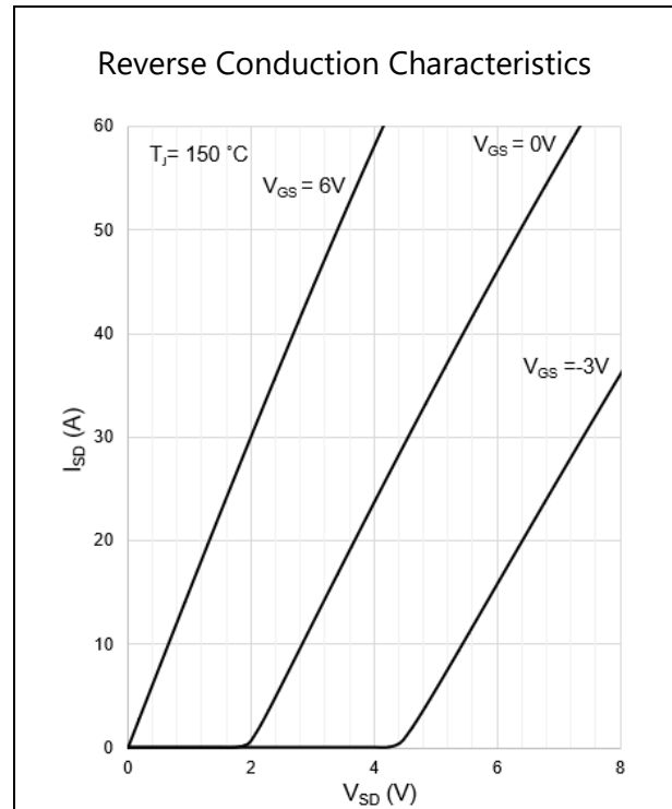
Figure 10: Typical I_{SD} vs. V_{SD} @ T_J = 150^\circ\text{C}
