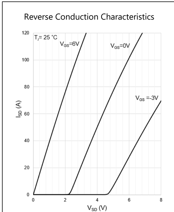
Figure 9: Typical I_{SD} vs. V_{SD} @ T_J = 25^\circ\text{C}
