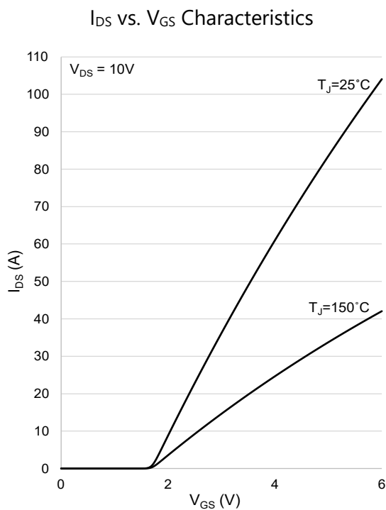
Figure 11: Typical I_{DS} vs. V_{GS}
