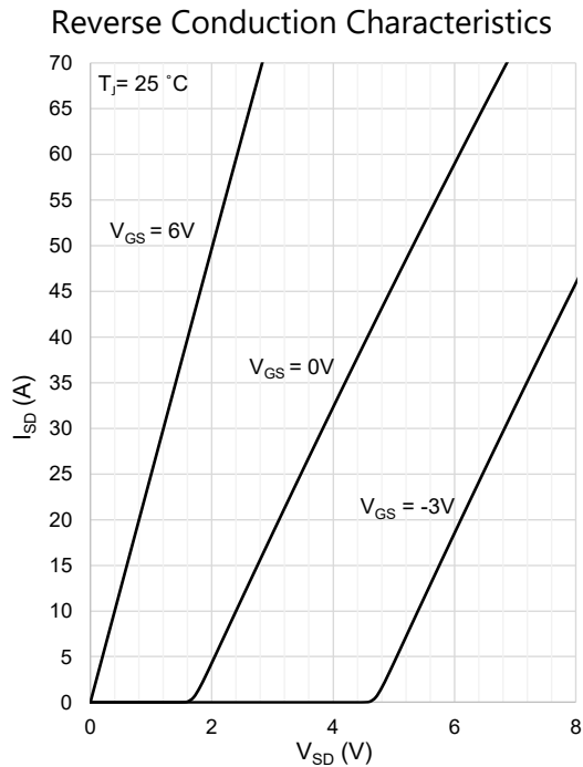
Figure 9: Typical I_{SD} vs. V_{SD} @ T_J = 25\text{ }^{\circ}\text{C}
