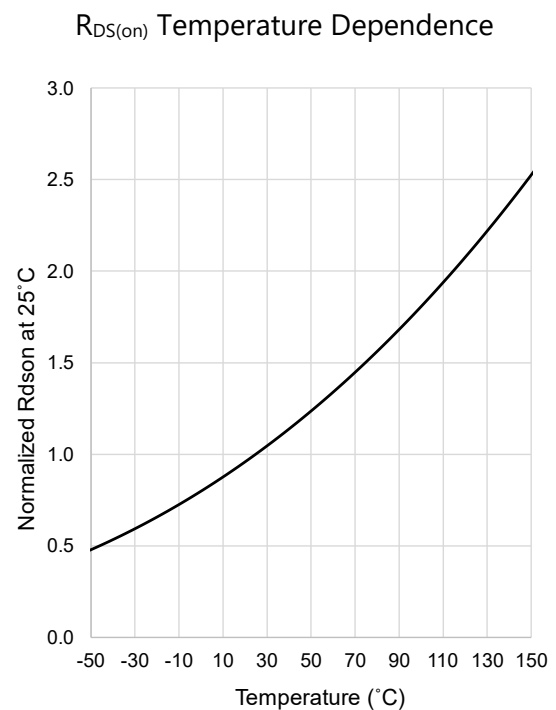
Figure 12: Normalized R_{DS(on)} as a function of T_J
