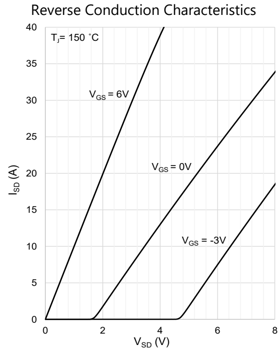
Figure 10: Typical I_{SD} vs. V_{SD} @ T_J = 150\text{ }^{\circ}\text{C}
