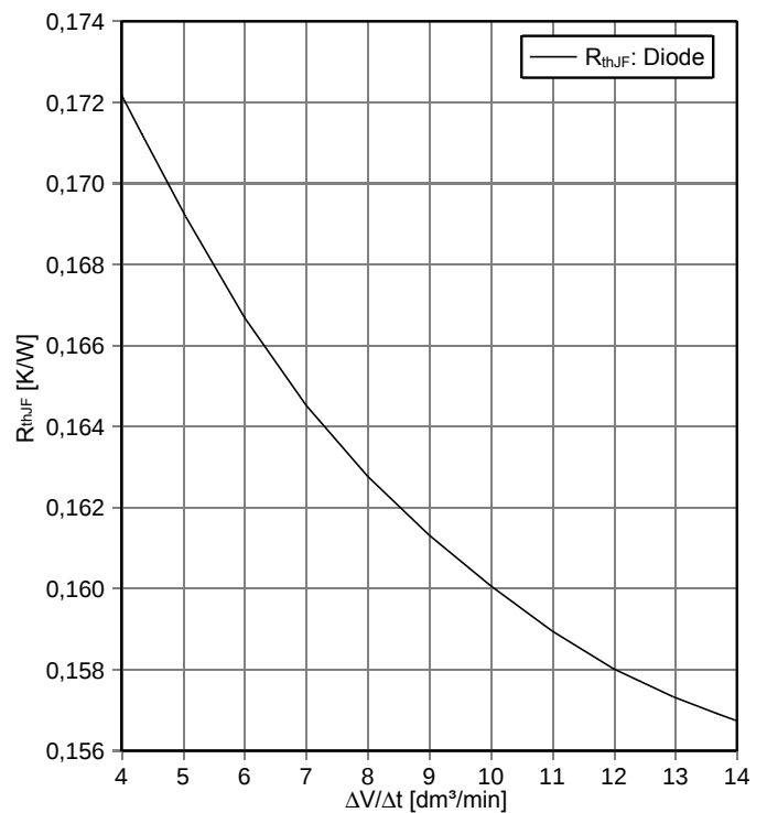
thermal impedance Diode, Inverter
