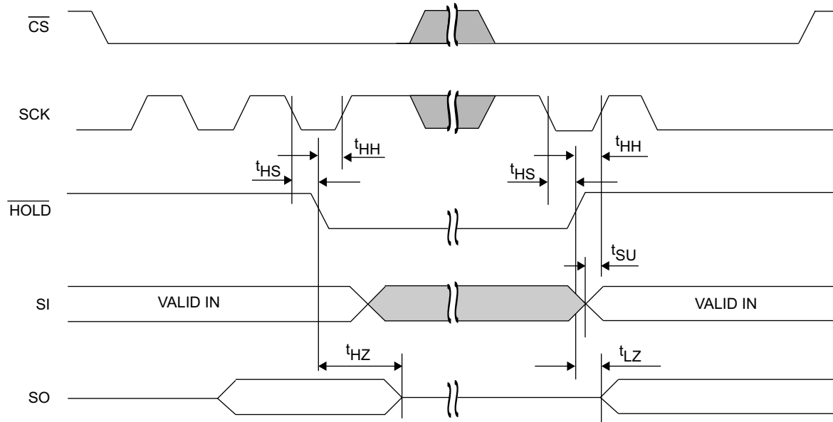
Figure 17. \overline{HOLD} Timing
