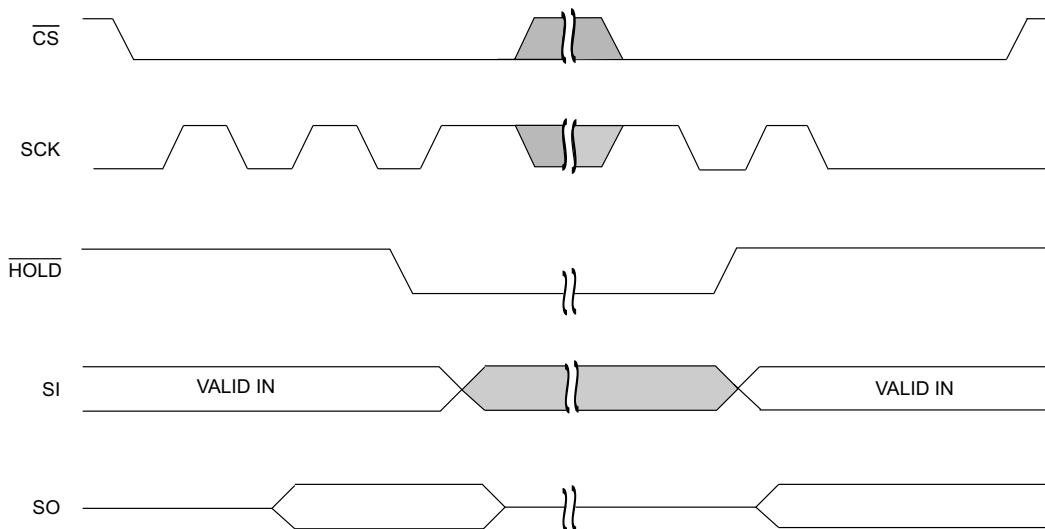
Figure 13. \overline{HOLD} Operation [2]
