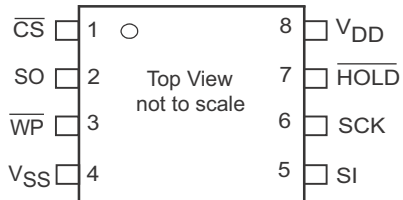
Figure 2. 8-pin TDFN pinout
