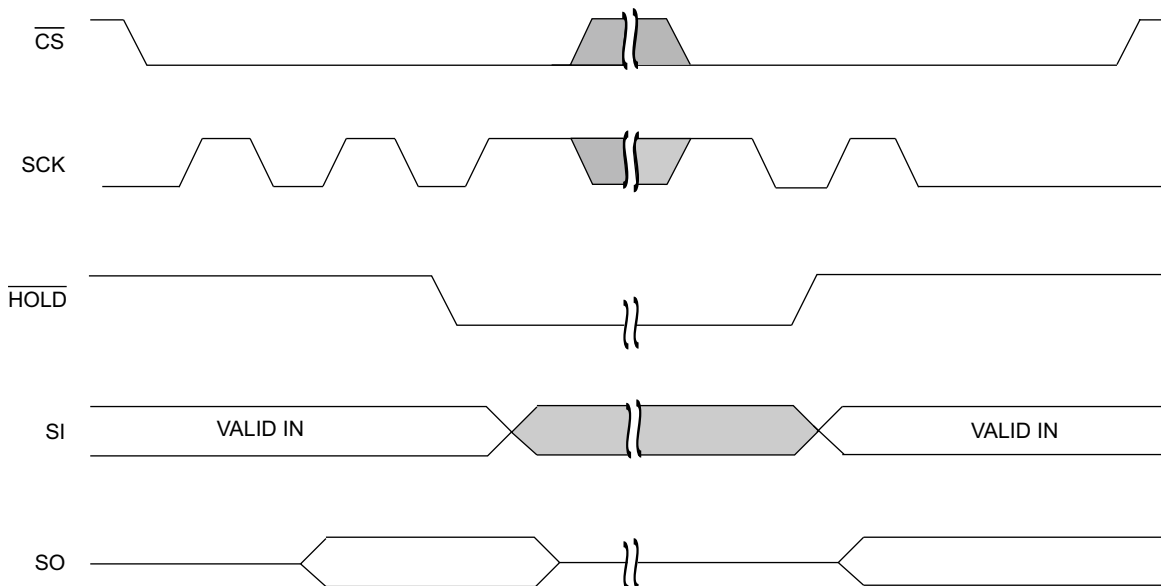
Figure 12. HOLD Operation [2]
