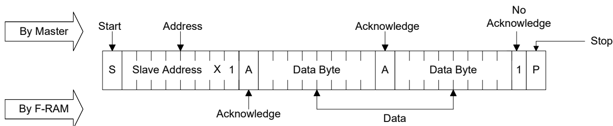
Figure 12. Sequential Read
