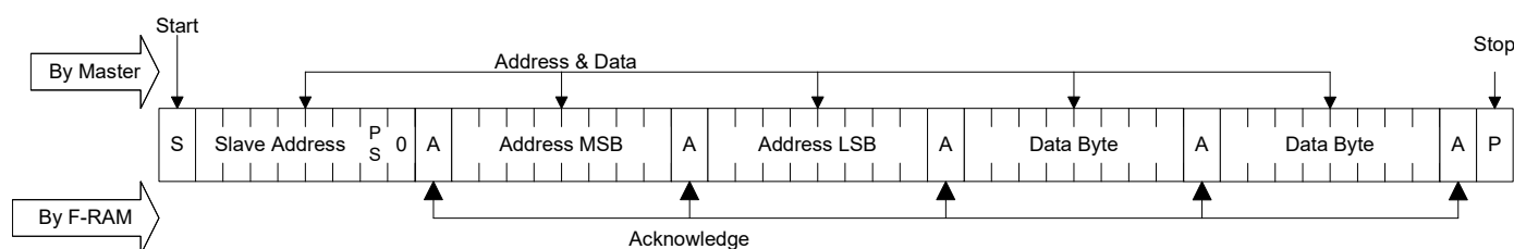
Figure 9. Multi-Byte Write
