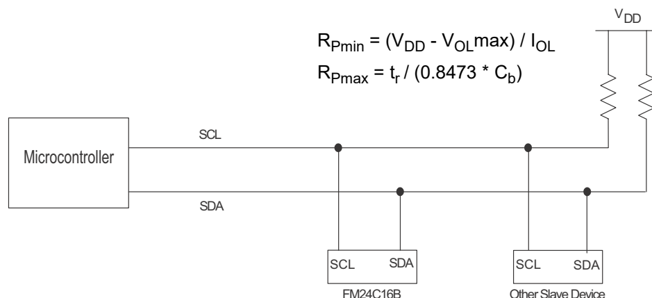
Figure 2. System Configuration using Serial (I 2 C) nvSRAM
