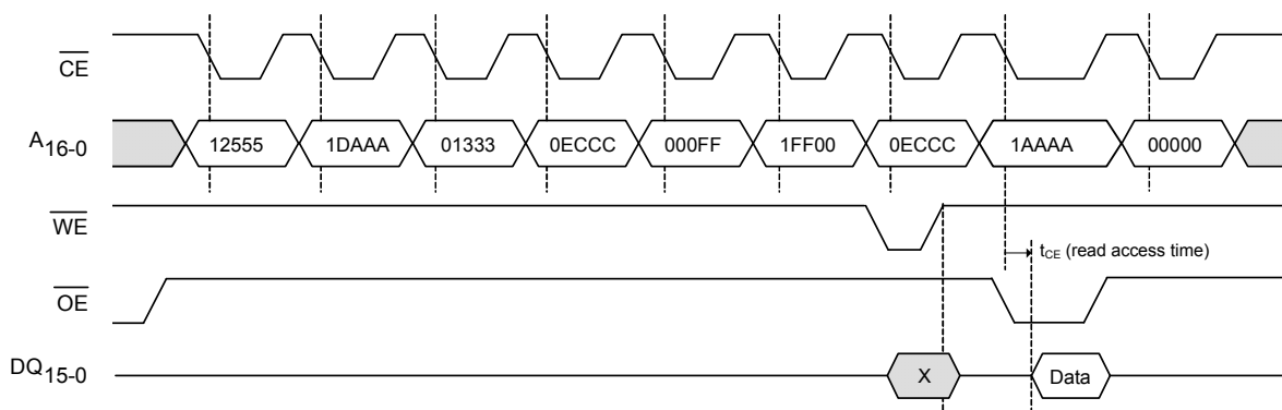
Figure 4. Sequence to Read Write-Protect Settings [1]
