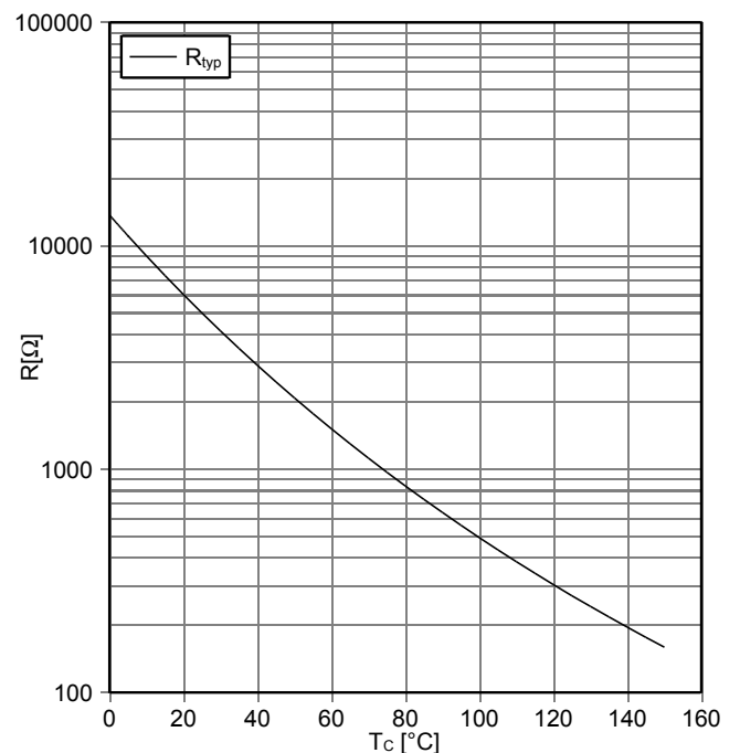
NTC-Thermistor-temperature characteristic (typical)
