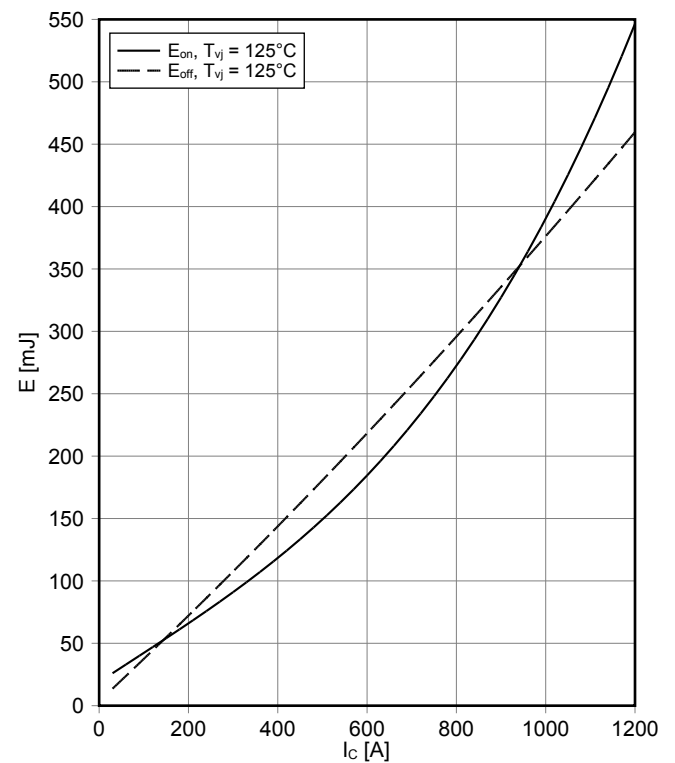
开关损耗 IGBT, 制动-斩波器 (典型) switching losses IGBT, Brake-Chopper (typical) E_{on} = f(I_C) , E_{off} = f(I_C) V_{GE} = \pm 15\text{ V} , R_{Gon} = 2.4\ \Omega , R_{Goff} = 3\ \Omega , V_{CE} = 900\text{ V}
