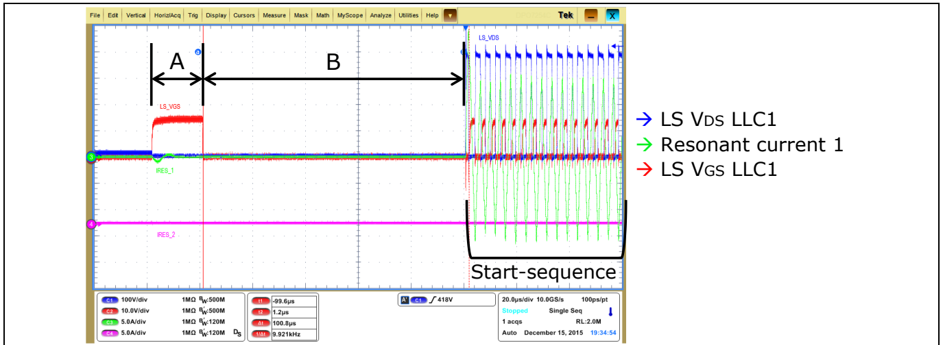
Figure 26 Pre-charge phase scope capture [Ch1=LS_Vds; Ch2=LS_Vgs; Ch3=Ires; Ch4=Ires2].
