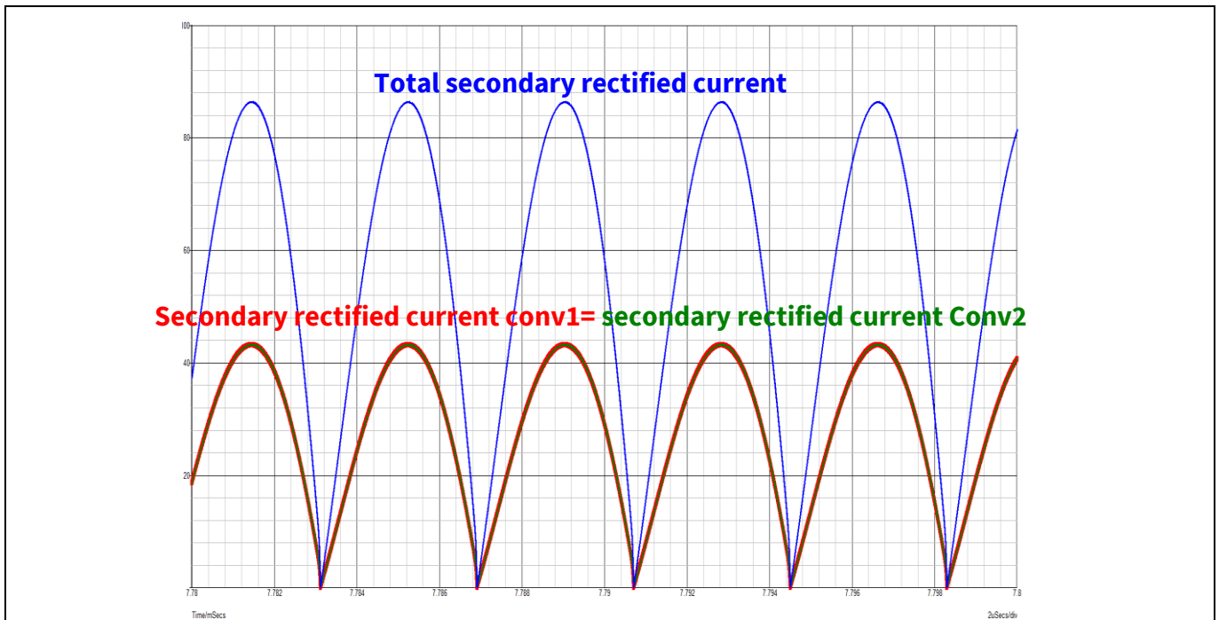
Figure 3 Secondary rectified currents in case of identical resonant tank components
