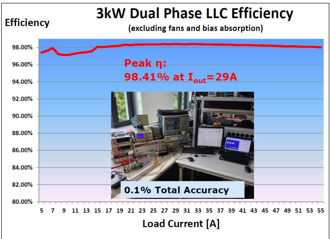
Figure 43 Efficiency versus Load measured with IPW60R040C7 at V_{in}=380V_{DC}
