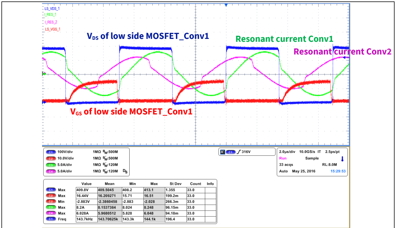
Figure 37 Resonant currents; V_{gs} and V_{ds} on the low side MOSFET (Conv1) at 50% load
