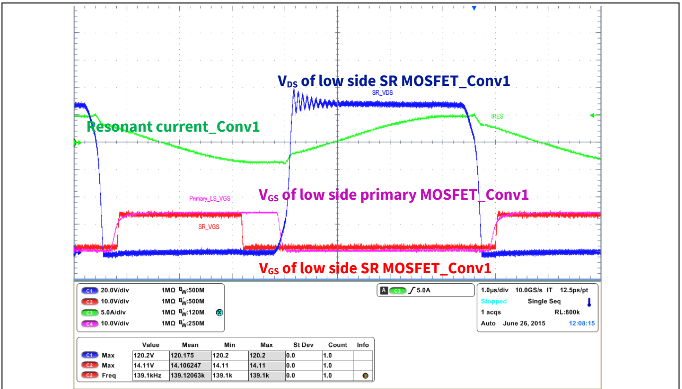
Figure 41 SR MOSFET operation at 10% load and V_{in} = 380 V_{DC} (Conv1)
