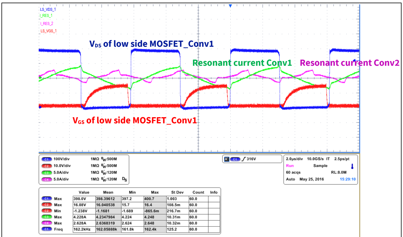
Figure 36 Resonant currents; V_{gs} and V_{ds} on the low side MOSFET (Conv1) at 10% load
