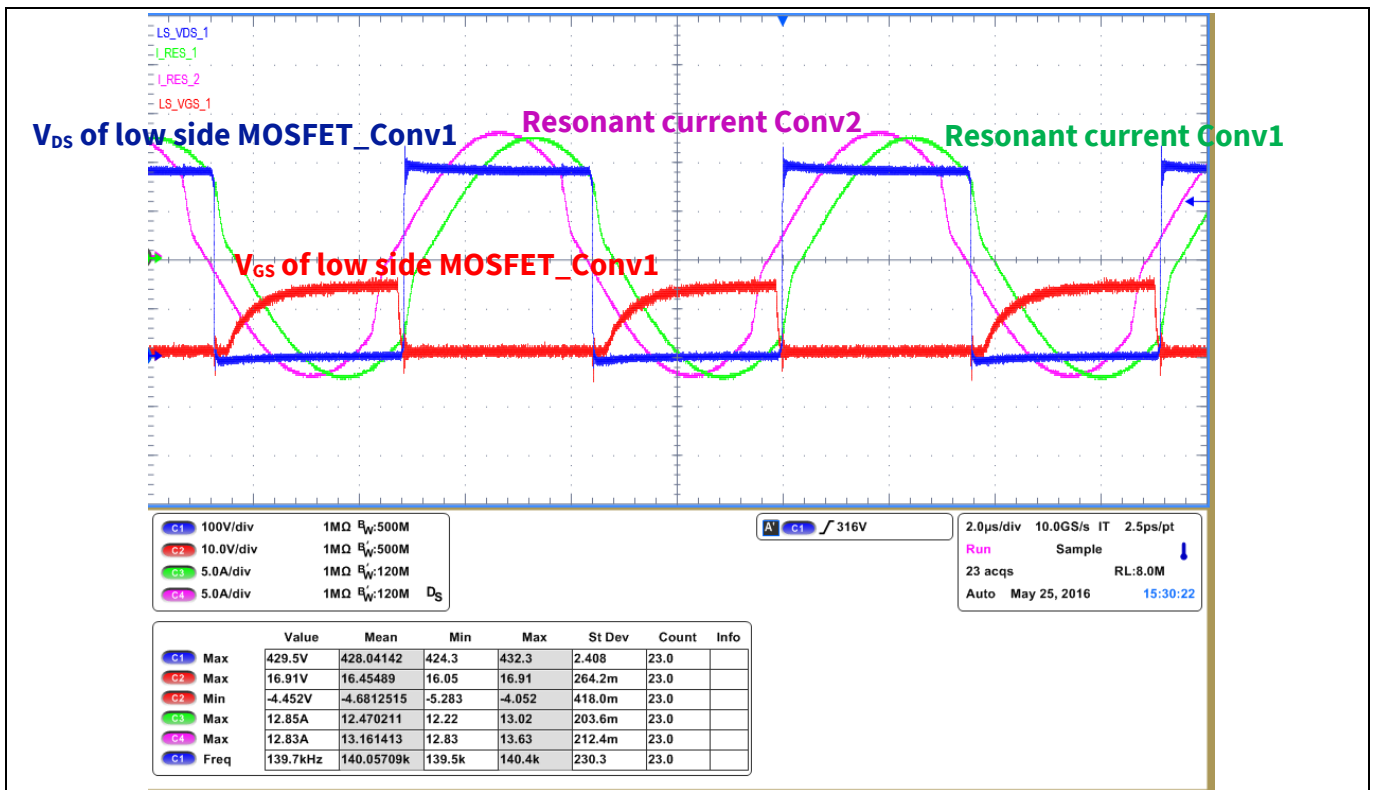
Figure 38 Resonant currents; V_{gs} and V_{ds} on the low side MOSFET (Conv1) at 100% load
