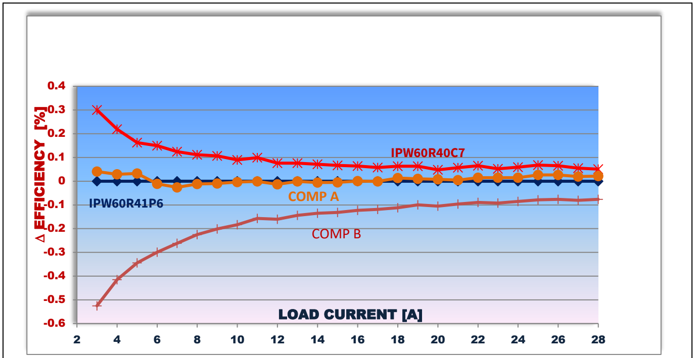
Figure 44 IPW60R040C7 versus IPW60R041P6 versus two competitors in 3 kW dual-phase LLC
