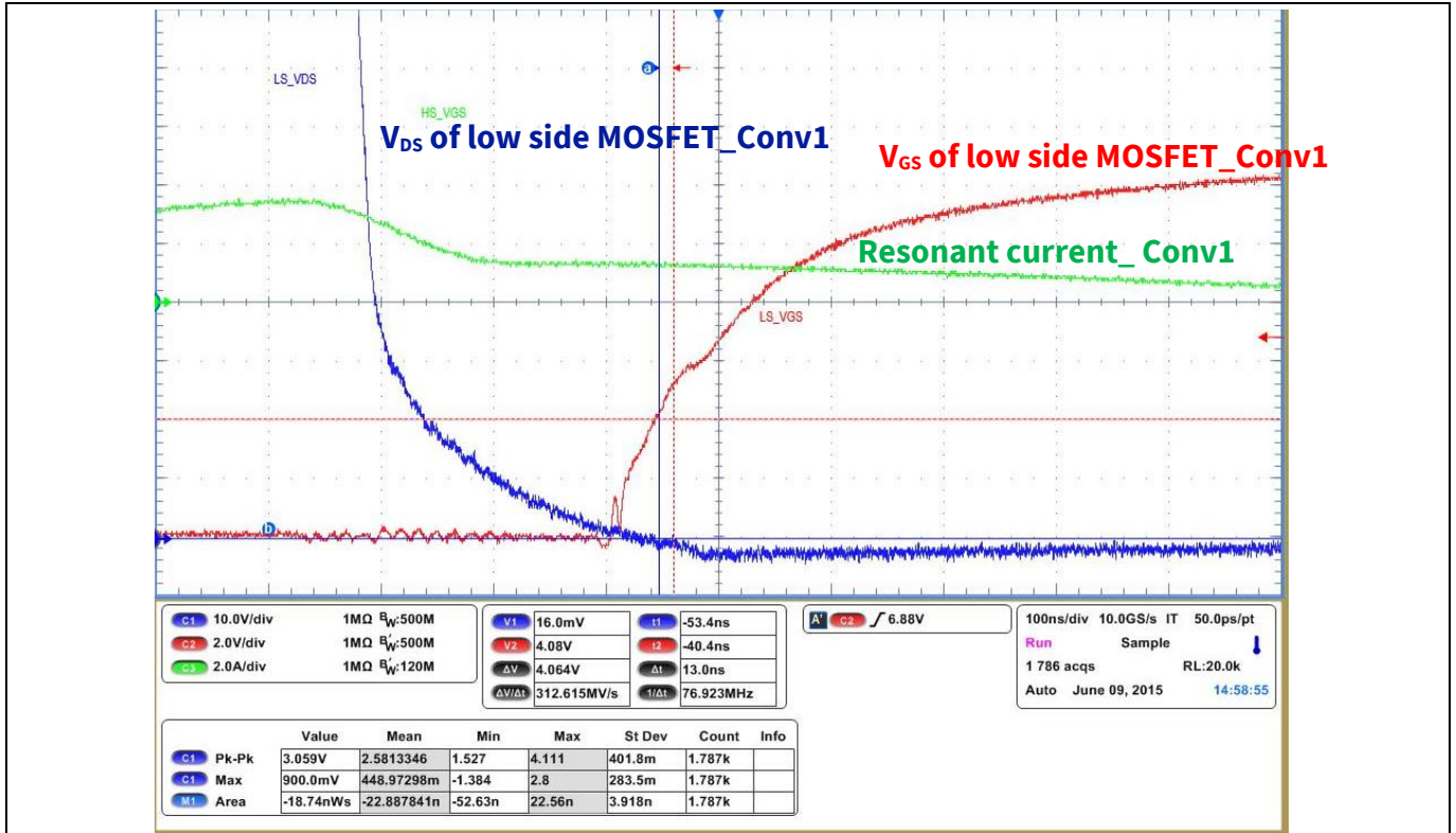
Figure 39 Full ZVS turn-on at only 3% load (90 W) and V_{in} = 380 V_{DC} (Conv1)
