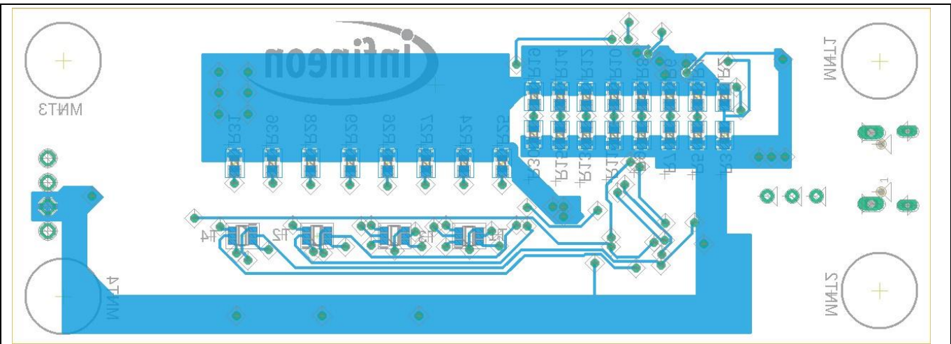
Figure 43 Bottom layer of DK_NLM_03
