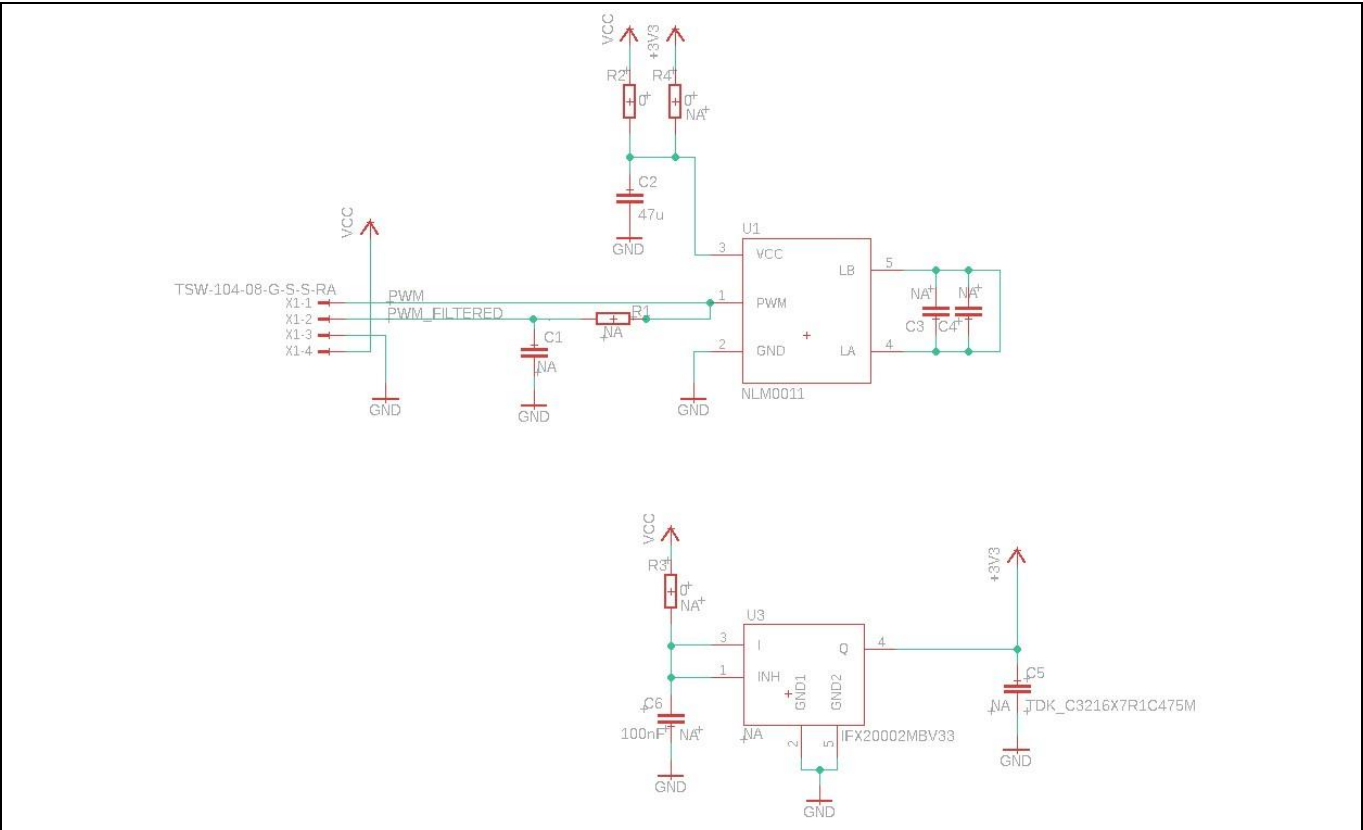
Figure 35 Schematic of NFC board DK_NLM_02
