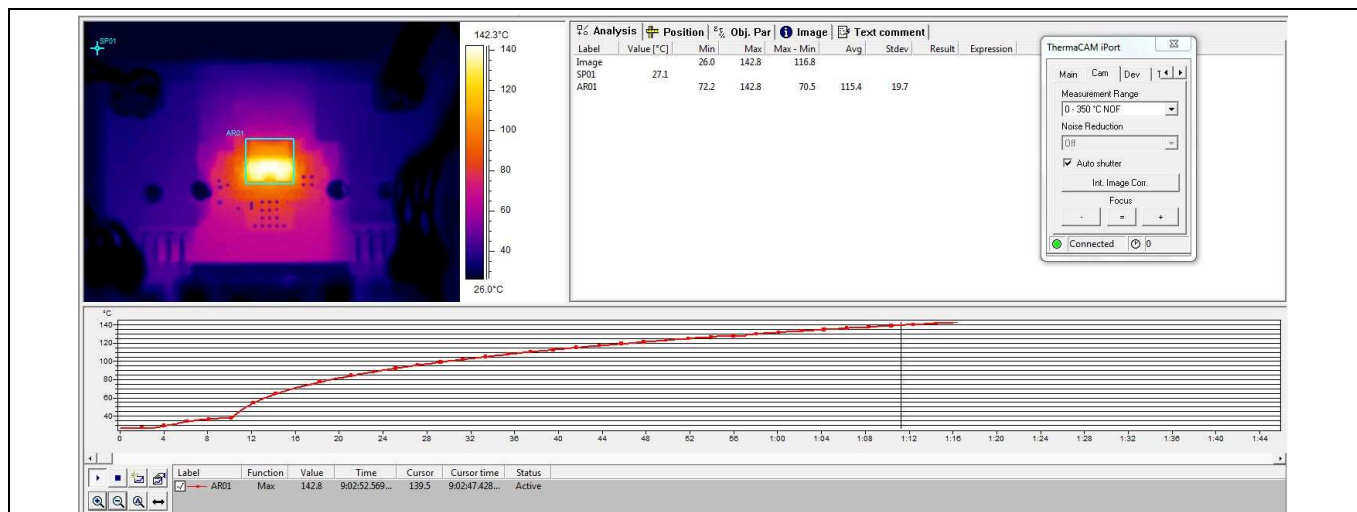
Figure 14 Peak power P_{out} = 55\text{ W} with 2\ \Omega load \pm 13.7\text{ V}
