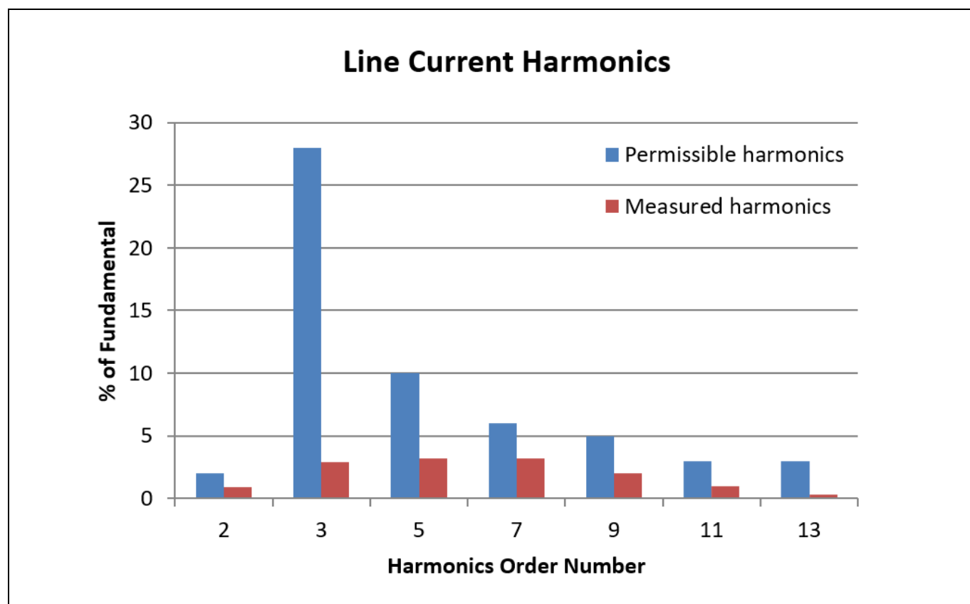
Figure 11 Line current harmonics V_{AC} = 230\text{ V}/60\text{ Hz} , 30% dimming
