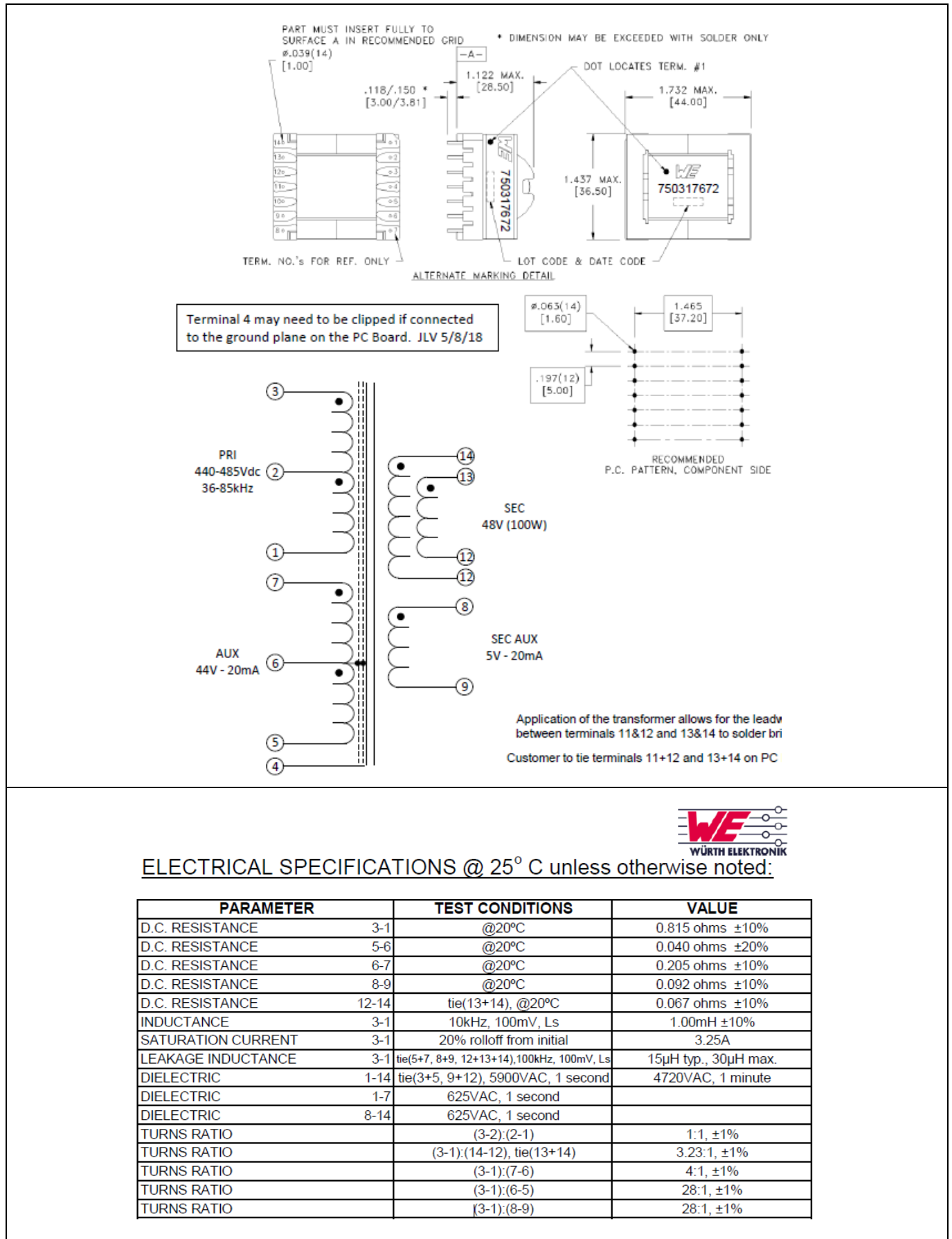
Figure 20 Würth Elektronik flyback transformer 750317672 rev00 specification
