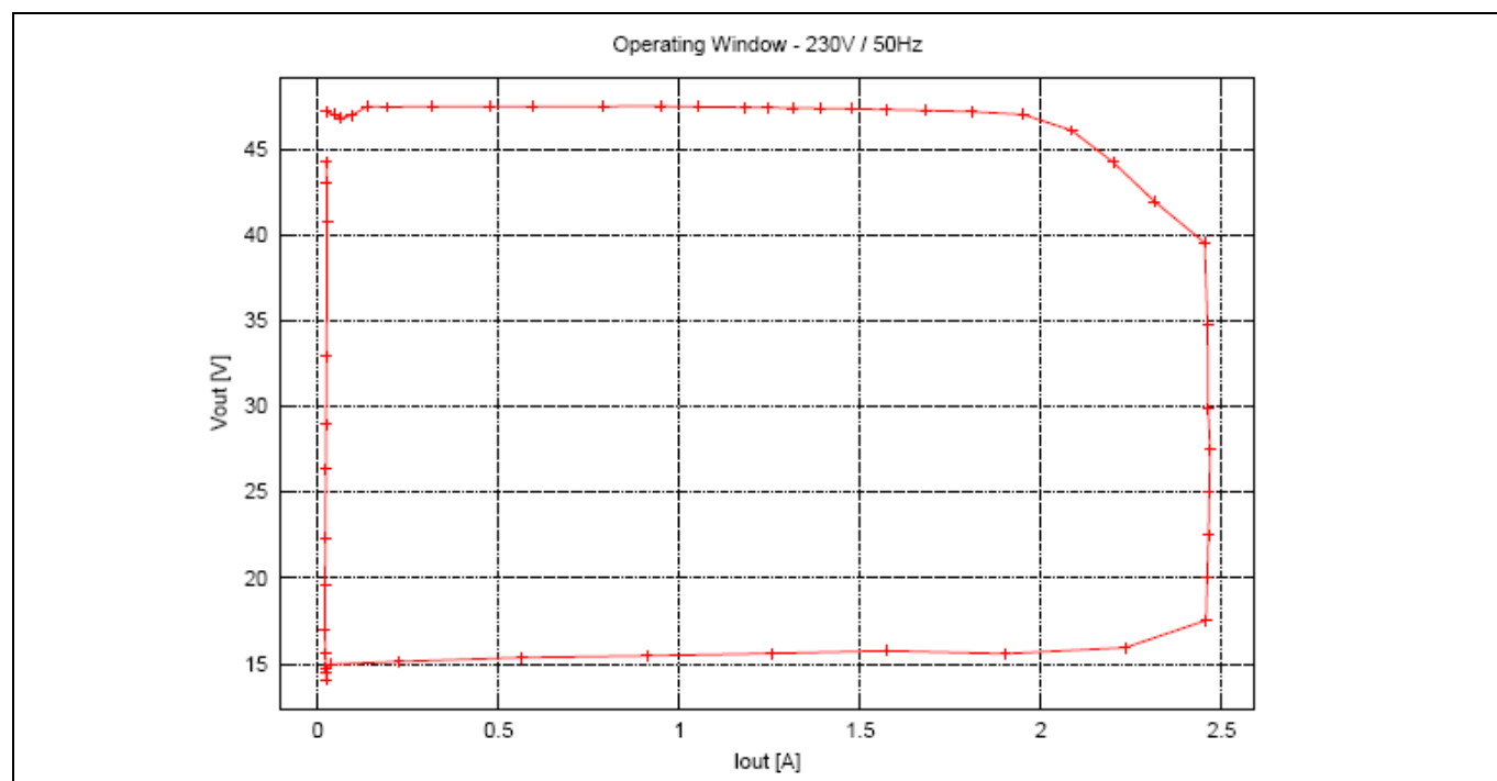
Figure 5 XDPL8221 100 W Reference board operating window
