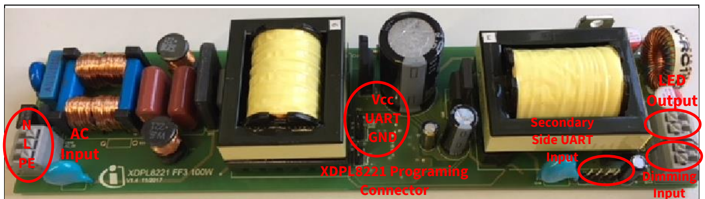
Figure 1 XDPL8221 100 W Reference board
