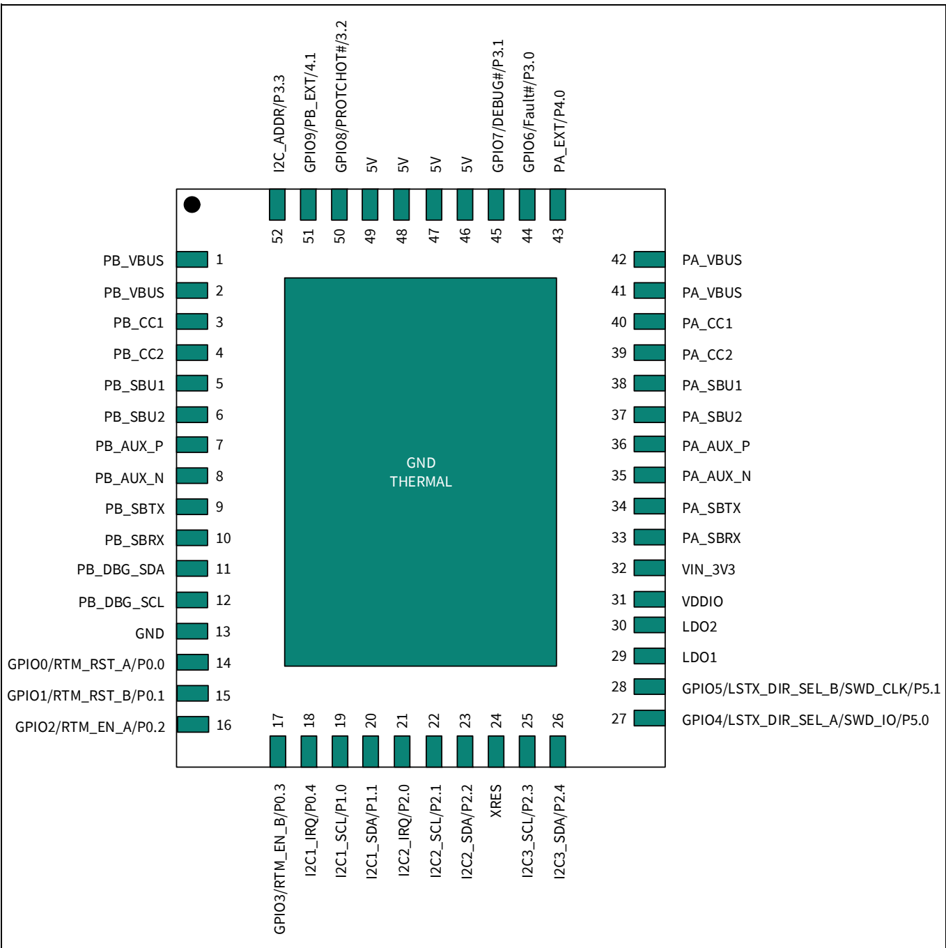
Figure 8 EZ-PD™ CCG8_CFP dual-port 52-lead QFN pinout
