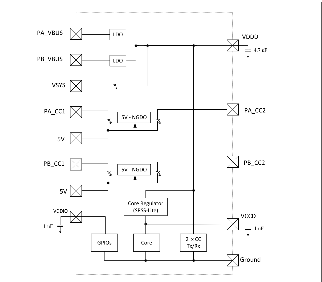
Figure 5 EZ-PD™ CCG8_CFP dual-port power system requirement block diagram
