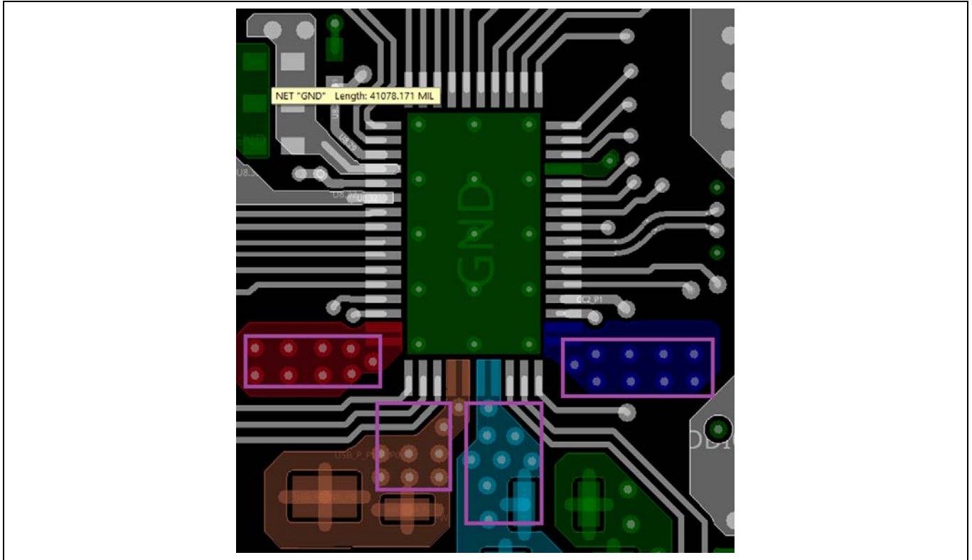
Figure 18 Via count for power pins
