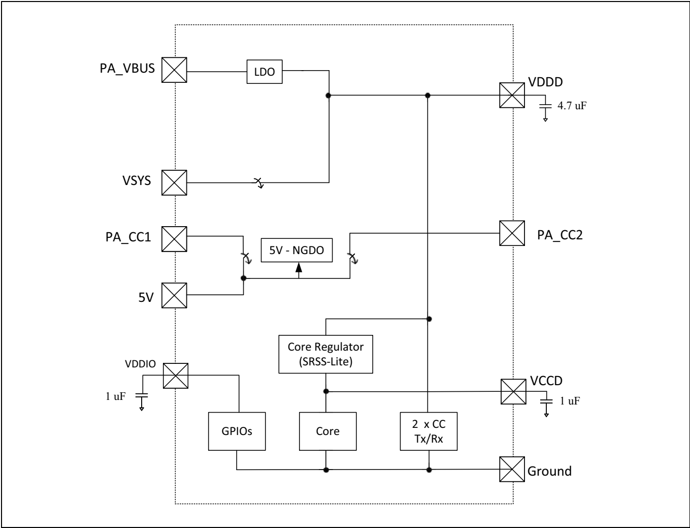
Figure 6 EZ-PD™ CCG8_CFP single-port power system requirement block diagram
