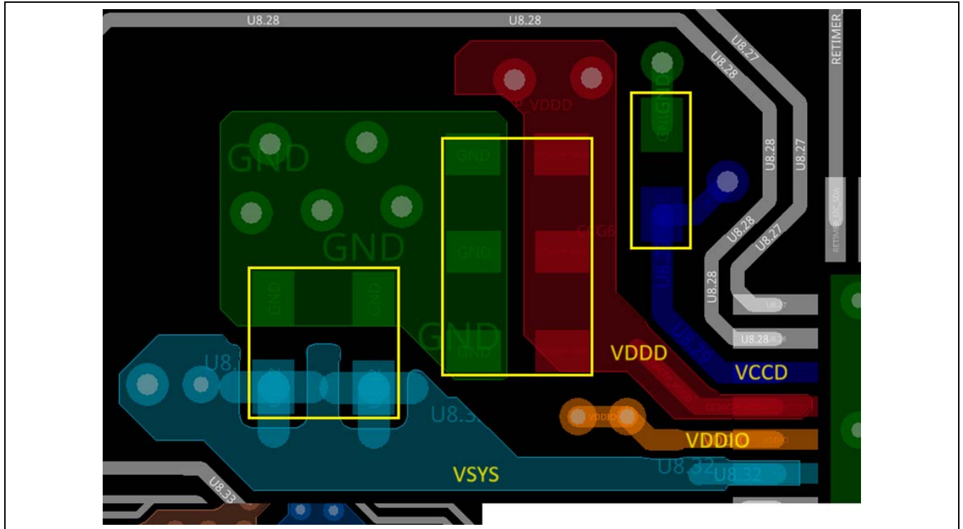
Figure 21 Top layer placement of caps
