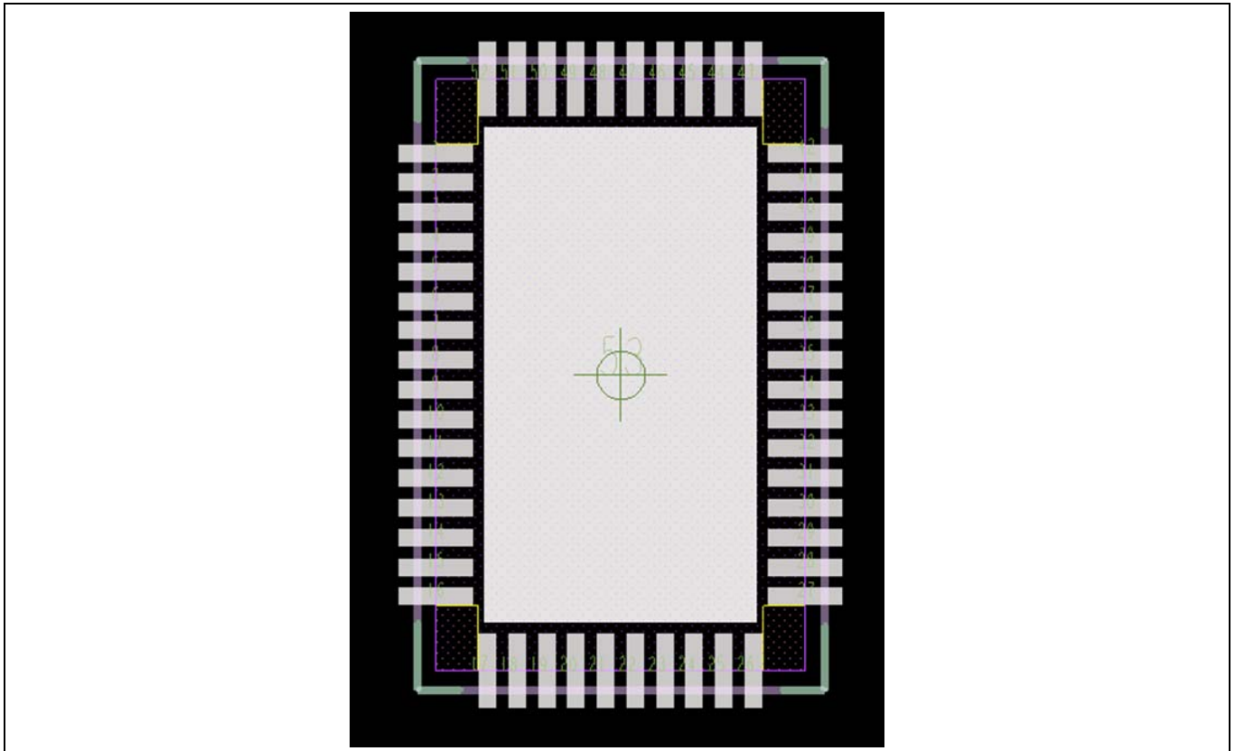
Figure 13 Top-view standard footprint (recommended) for CCG8_CFP
