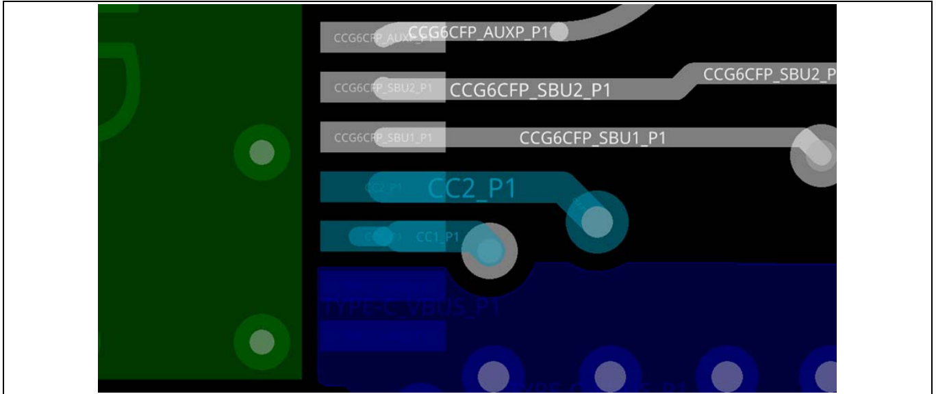
Figure 19 CC1 and CC2 fanout (showing Port 1)
