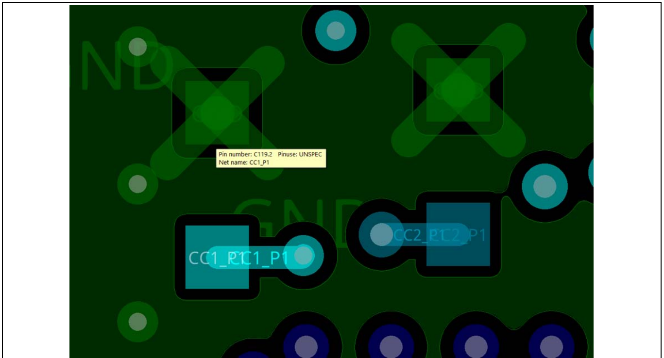
Figure 20 CC1 and CC2 caps
