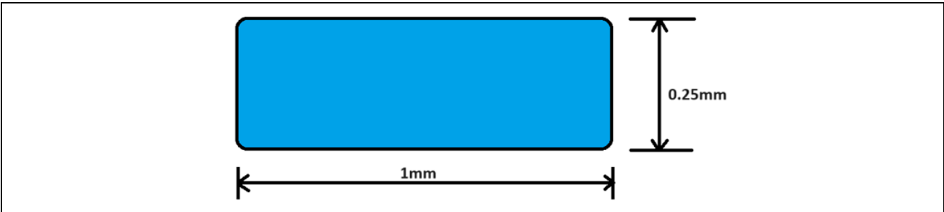
Figure 14 QFN pad size
