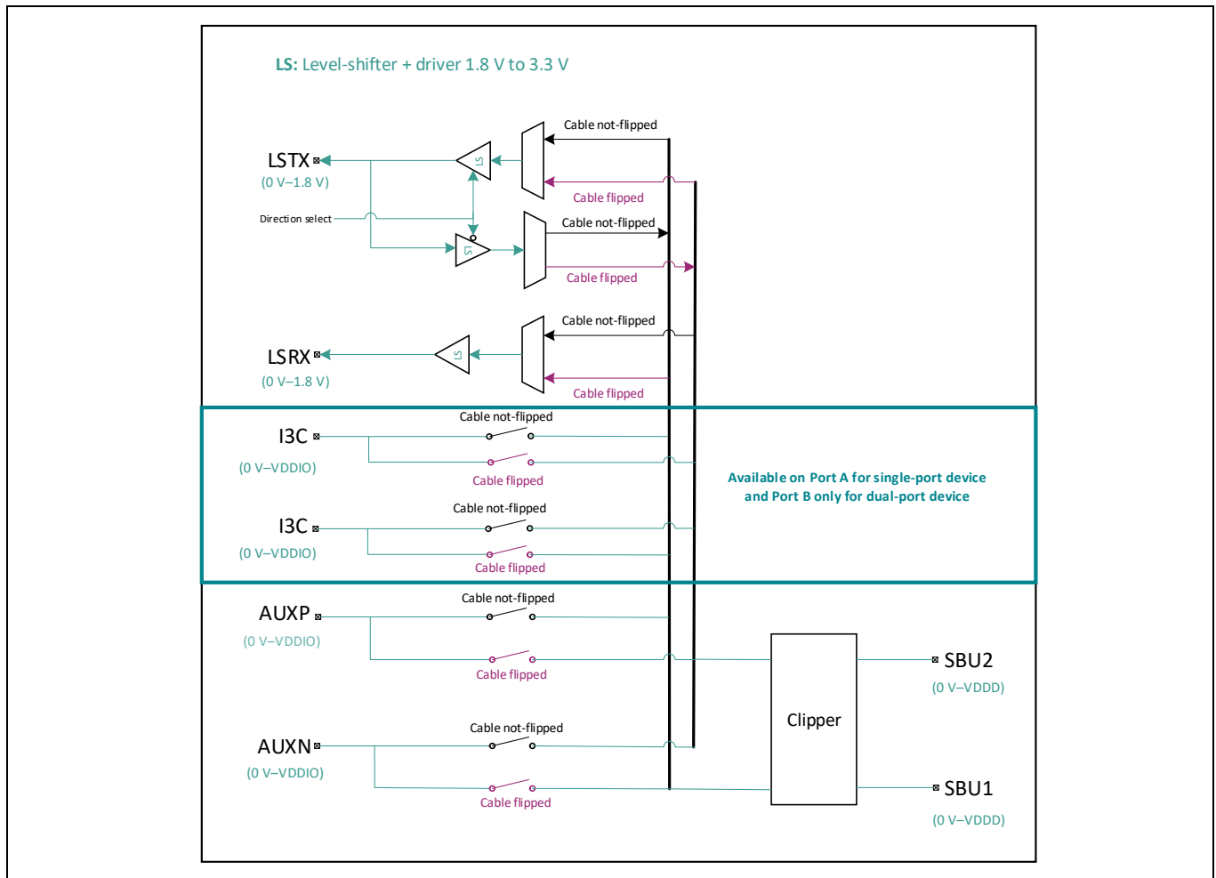
Figure 3 High-speed crossbar switch internal block diagram
