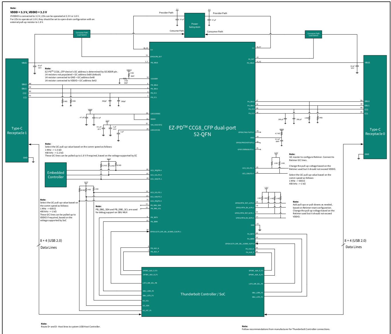
Figure 11 EZ-PD™ CCG8_CFP dual-port application block diagram with VDDIO = 3.3 V
