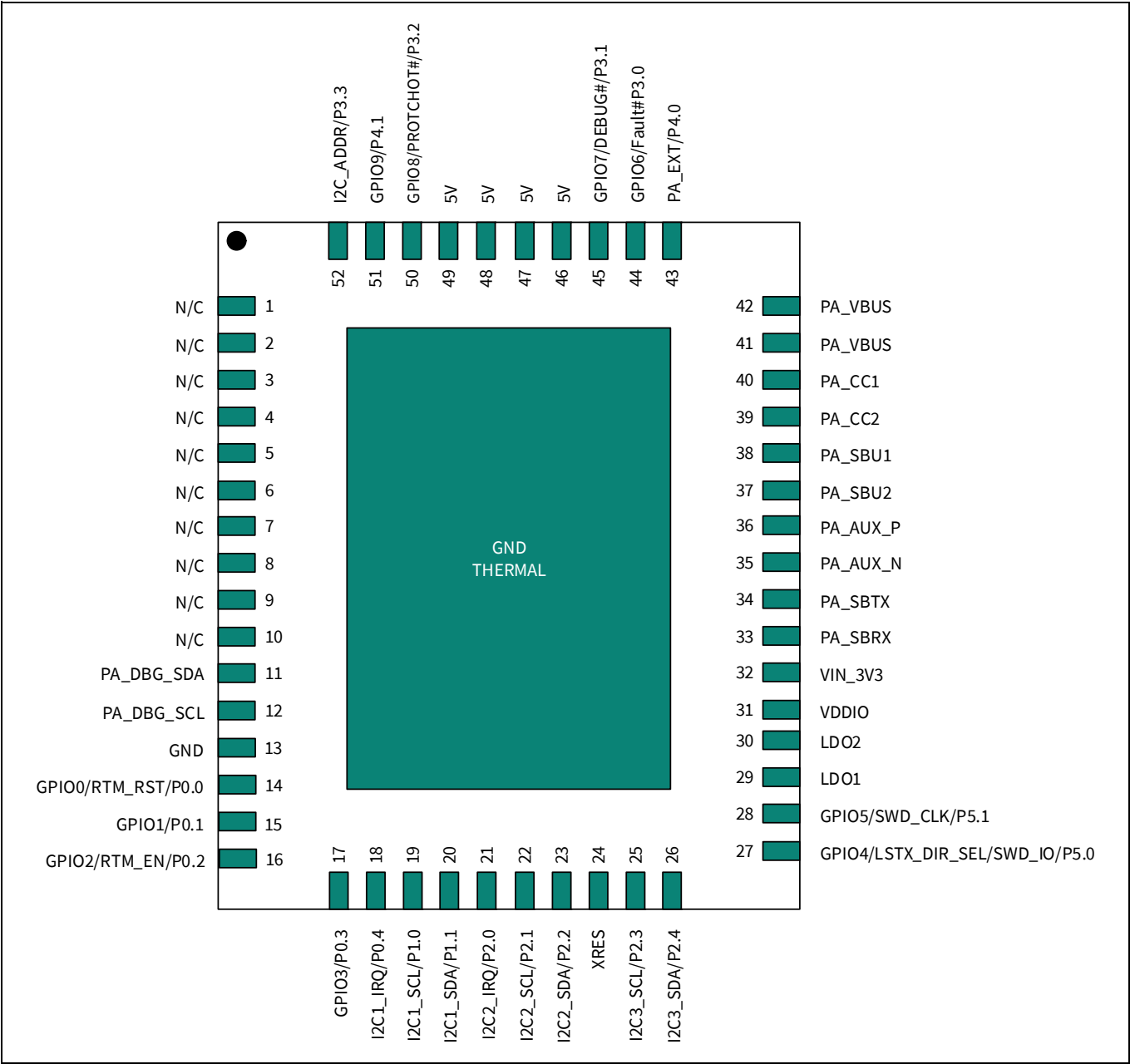
Figure 7 EZ-PD™ CCG8_CFP single-port 52-lead QFN pinout
