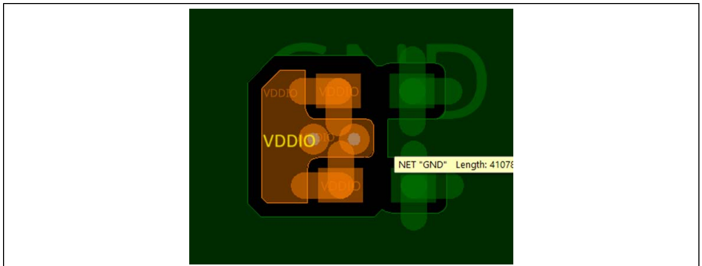
Figure 22 Bottom layer placement of VDDIO caps
