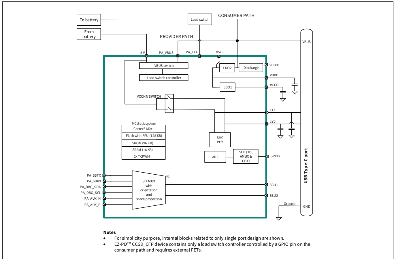
Figure 1 EZ-PD™ CCG8_CFP functional block diagram for single-port device
