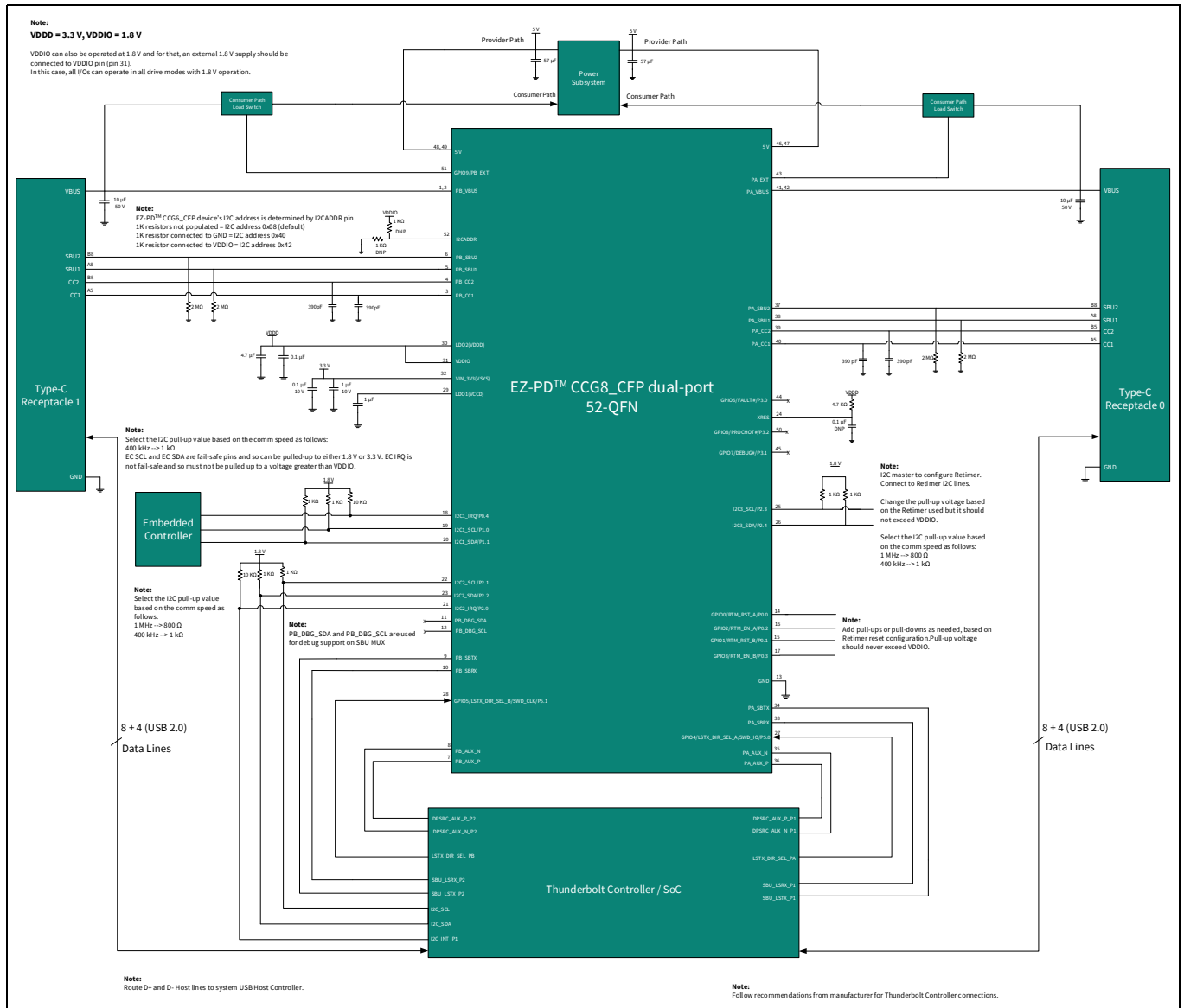
Figure 12 EZ-PD™ CCG8_CFP dual-port application block diagram with VDDIO = 1.8 V
