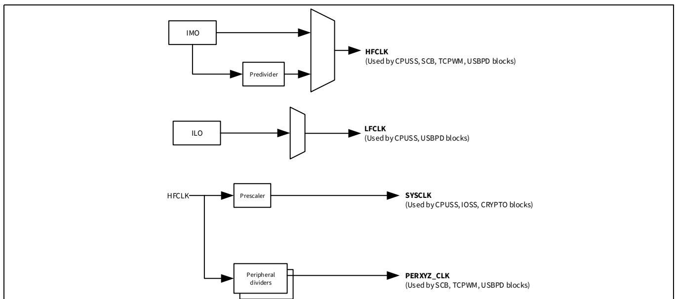
Figure 4 EZ-PD™ CCG8_CFP clocking architecture
