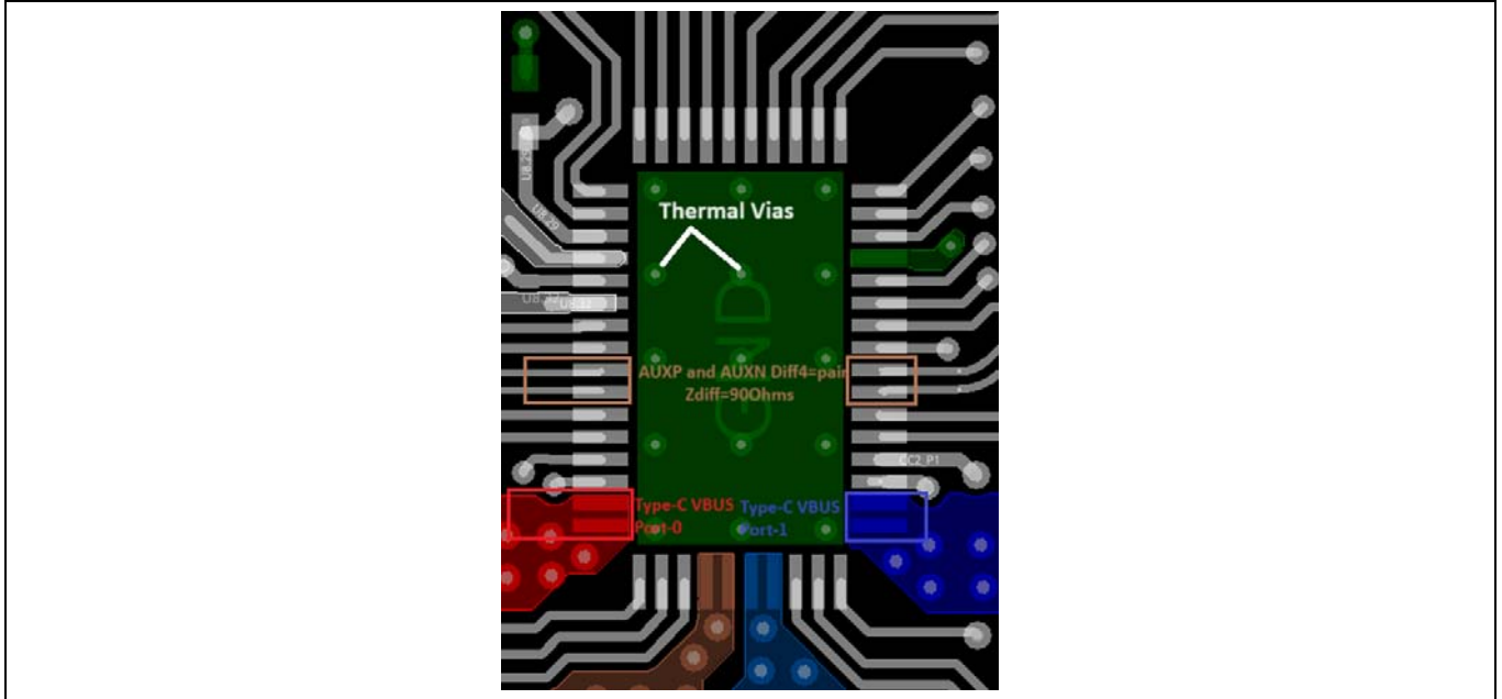
Figure 16 QFN fanout with thermal vias
