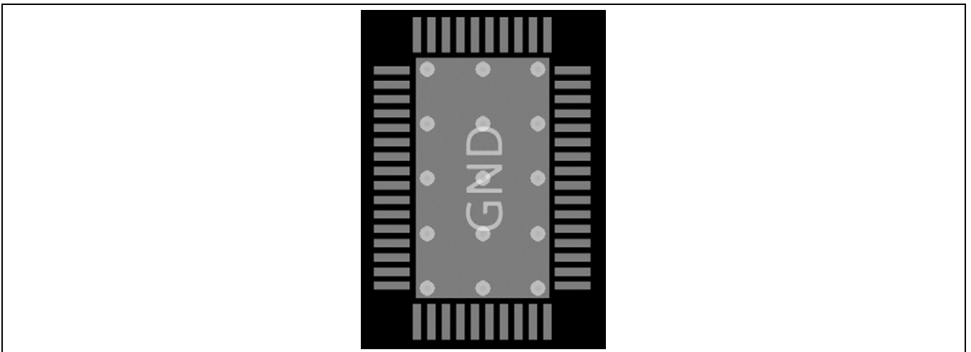
Figure 17 Thermal pad (EPAD) and thermal via
