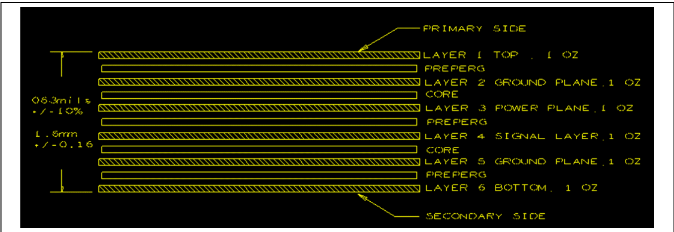
Figure 15 Six-layer stack-up
