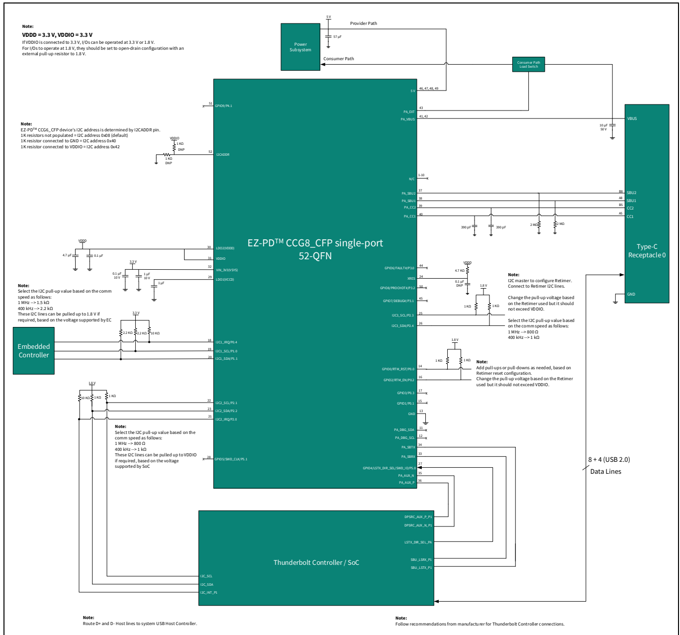
Figure 9 EZ-PD™ CCG8_CFP single-port application block diagram with VDDIO = 3.3 V
