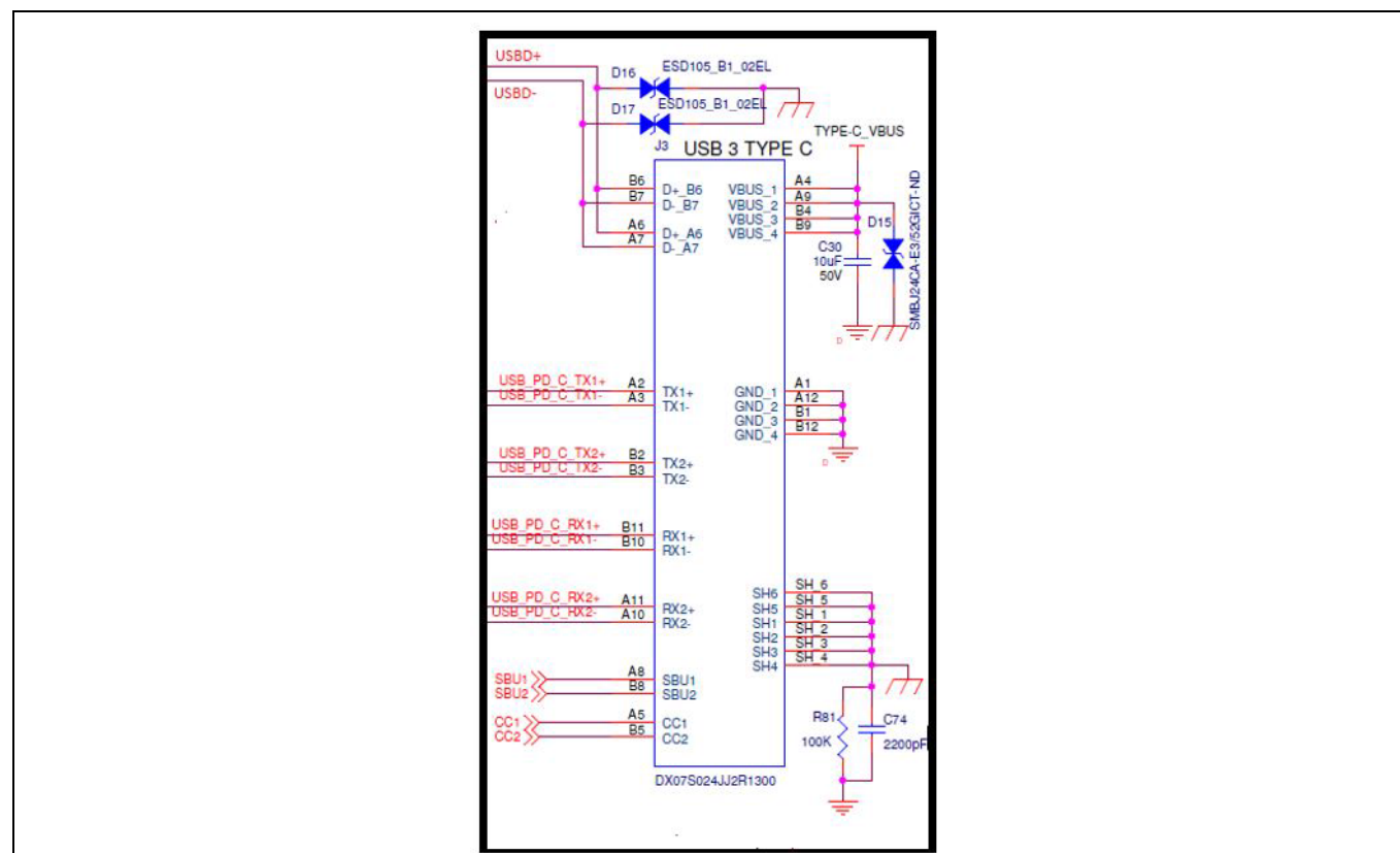
Figure 5 ESD and EMC protection
