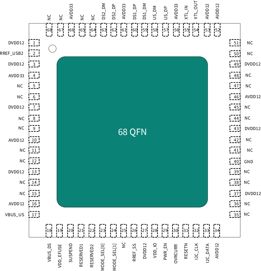
Figure 11 68-pin QFN pinout for CYUSB2304
