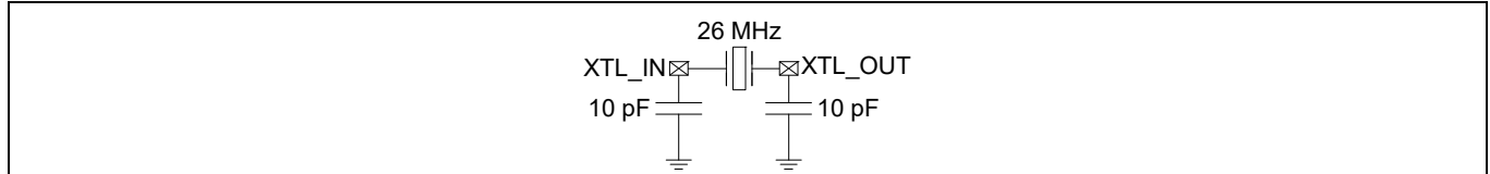
Figure 15 Crystal connection
