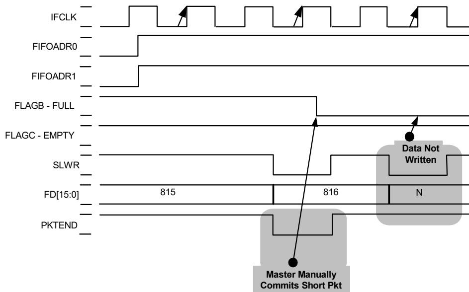
Figure 9-14. Timing Example: Synchronous FIFO Writes, Waveform 3, PKTEND Pin Illustrated
