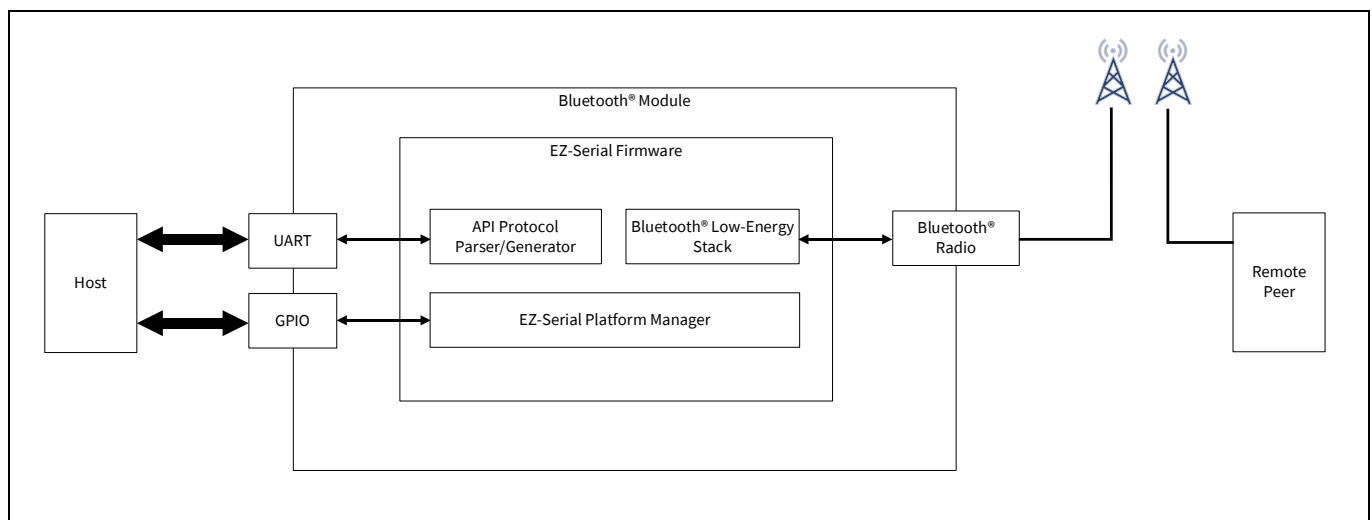
Figure 1 EZ-Serial system block diagram
