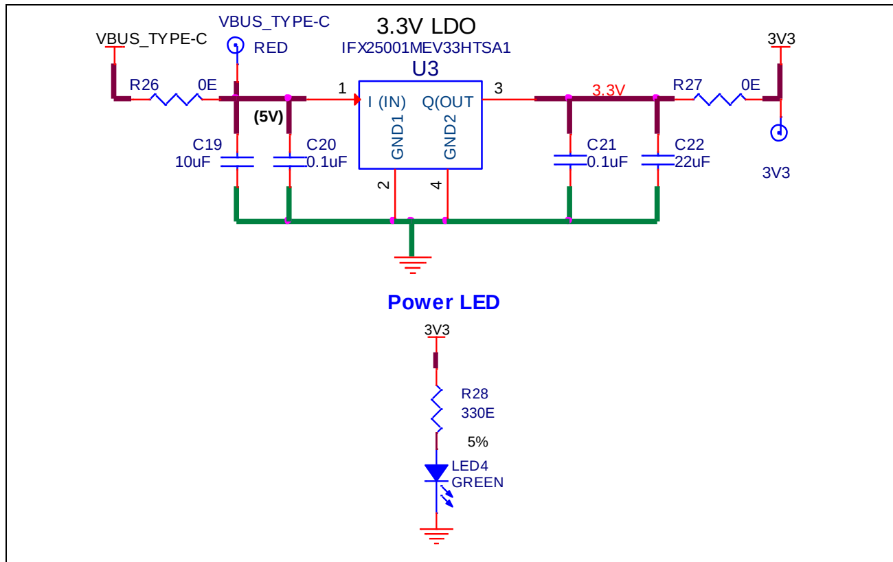
Figure 21 Onboard 3.3-V LDO and power LED
