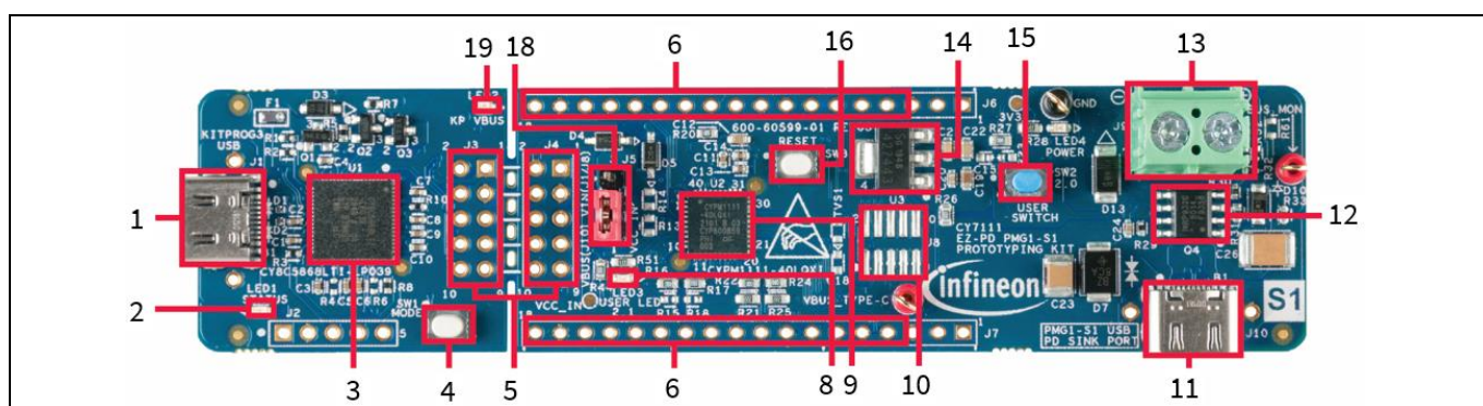
Figure 3 CY7111 EZ-PD™ PMG1-S1 MCU prototyping kit
