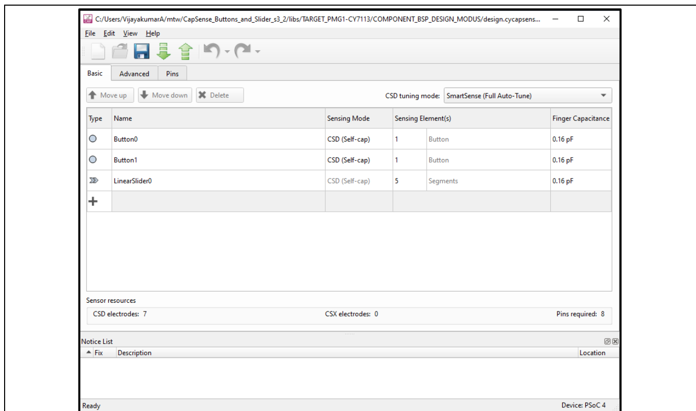
Figure 16 CAPSENSE™ configurator
