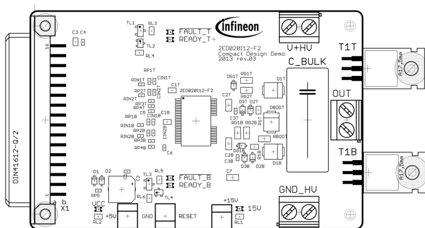
Figure 4-8 top place view of the EVAL_2ED020I12-F2
