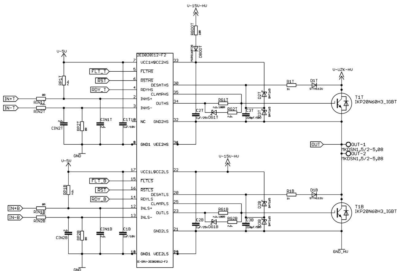
Figure 4-4 Infineon driver 2ED020I12-F2 top and bottom
