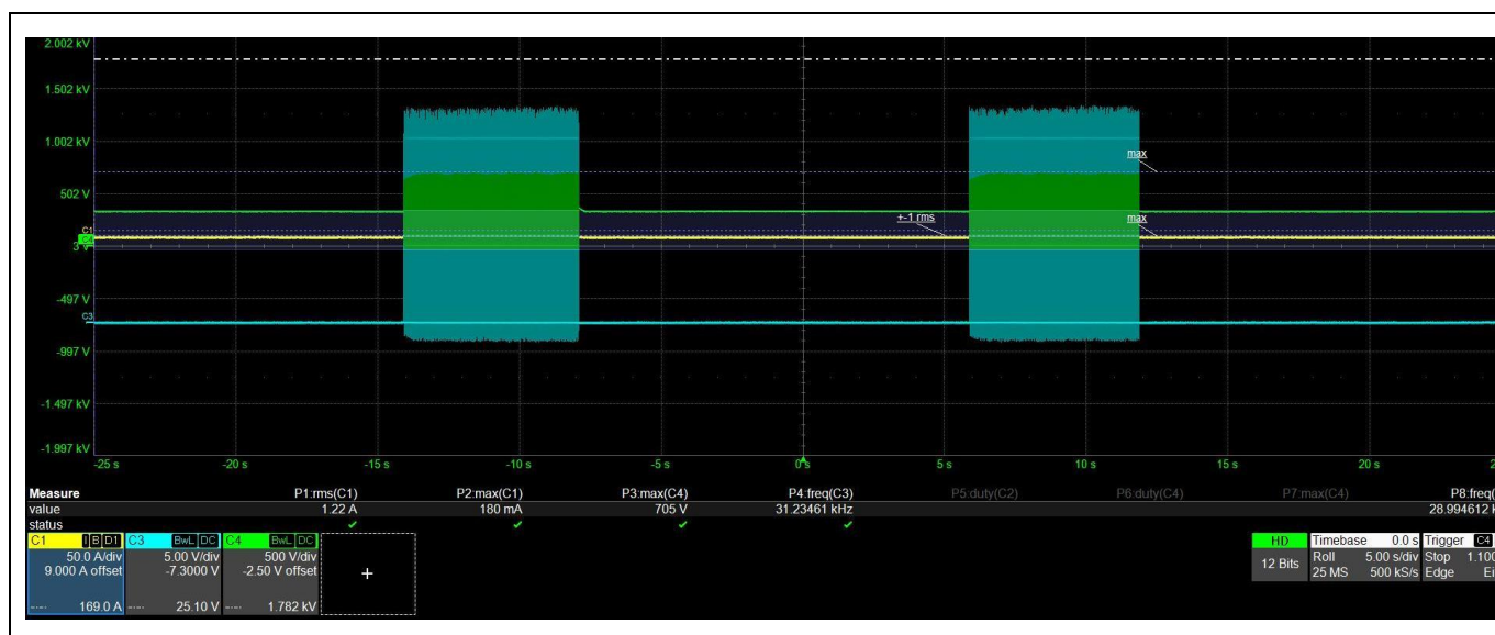
Figure 15 Burst mode operation at power level 3
