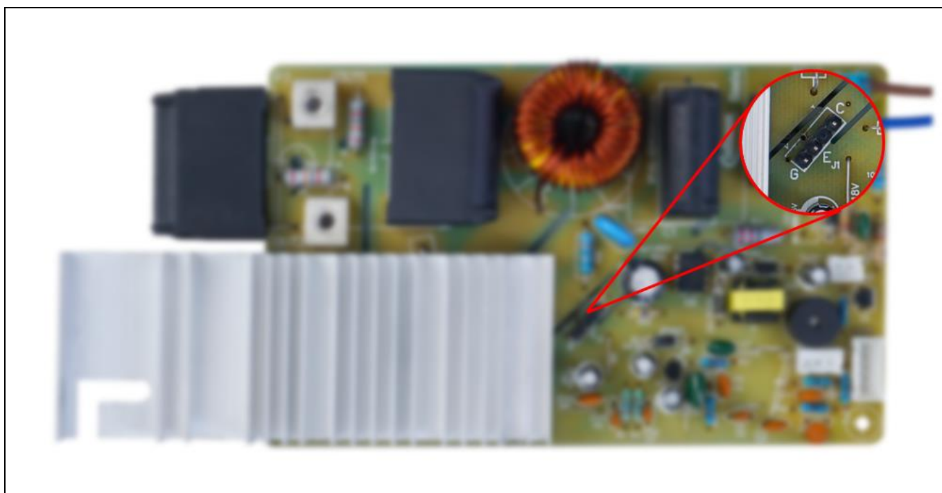
Figure 9 IGBT test points
