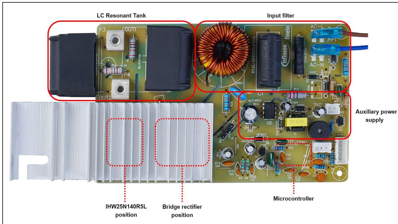
Figure 3 Quasi-resonant board: building blocks
