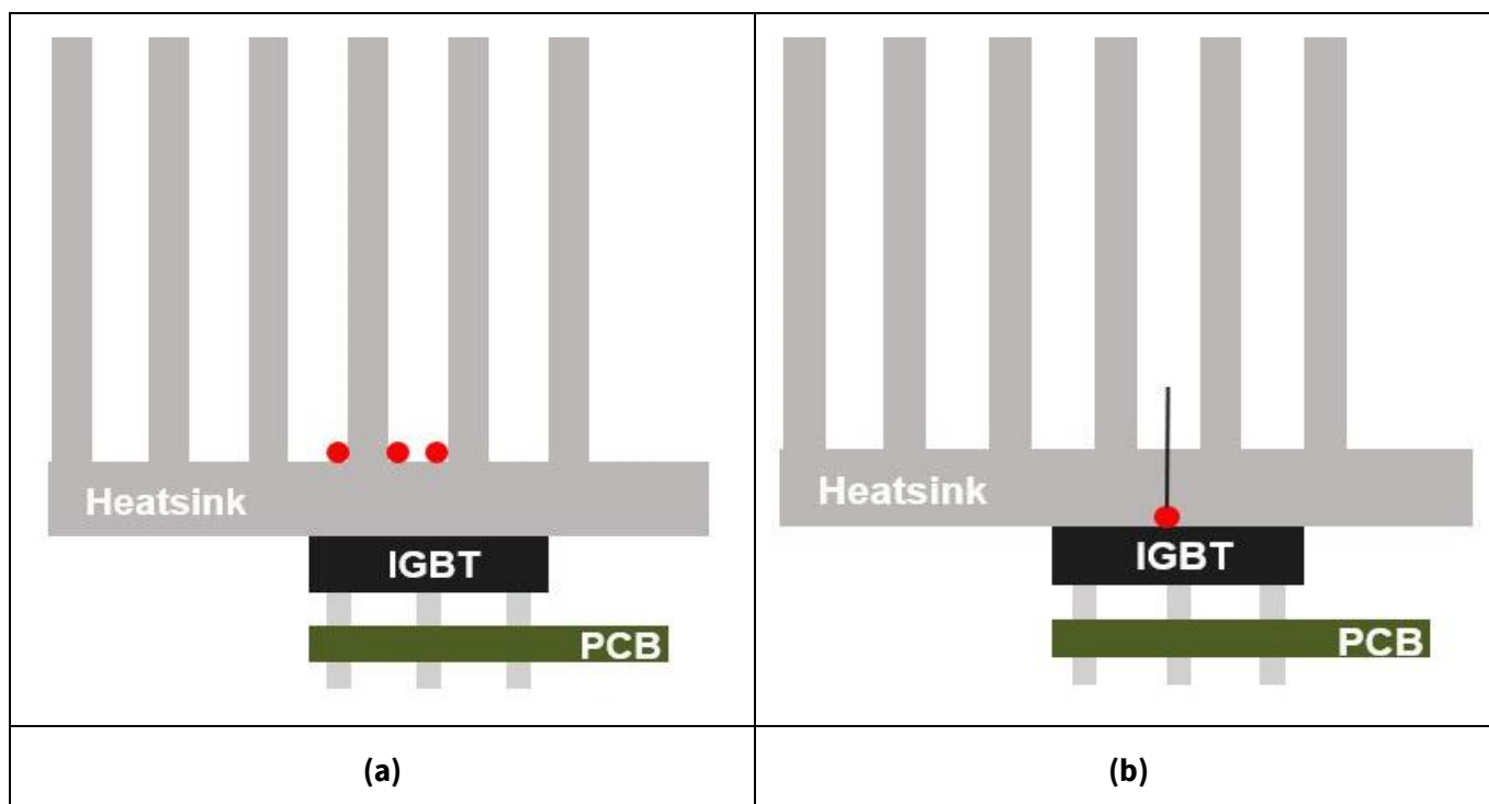
Figure 11 Recommended mounting for the thermocouple
