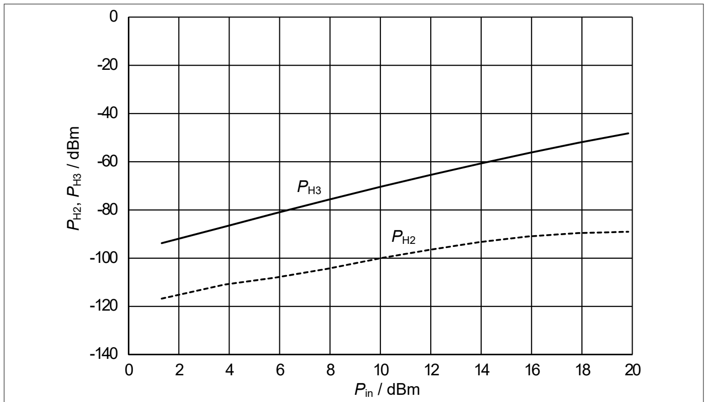
Figure 12 Second and third harmonic power: P_{H2}, P_{H3} = f(P_{in}) at f = 900 MHz
