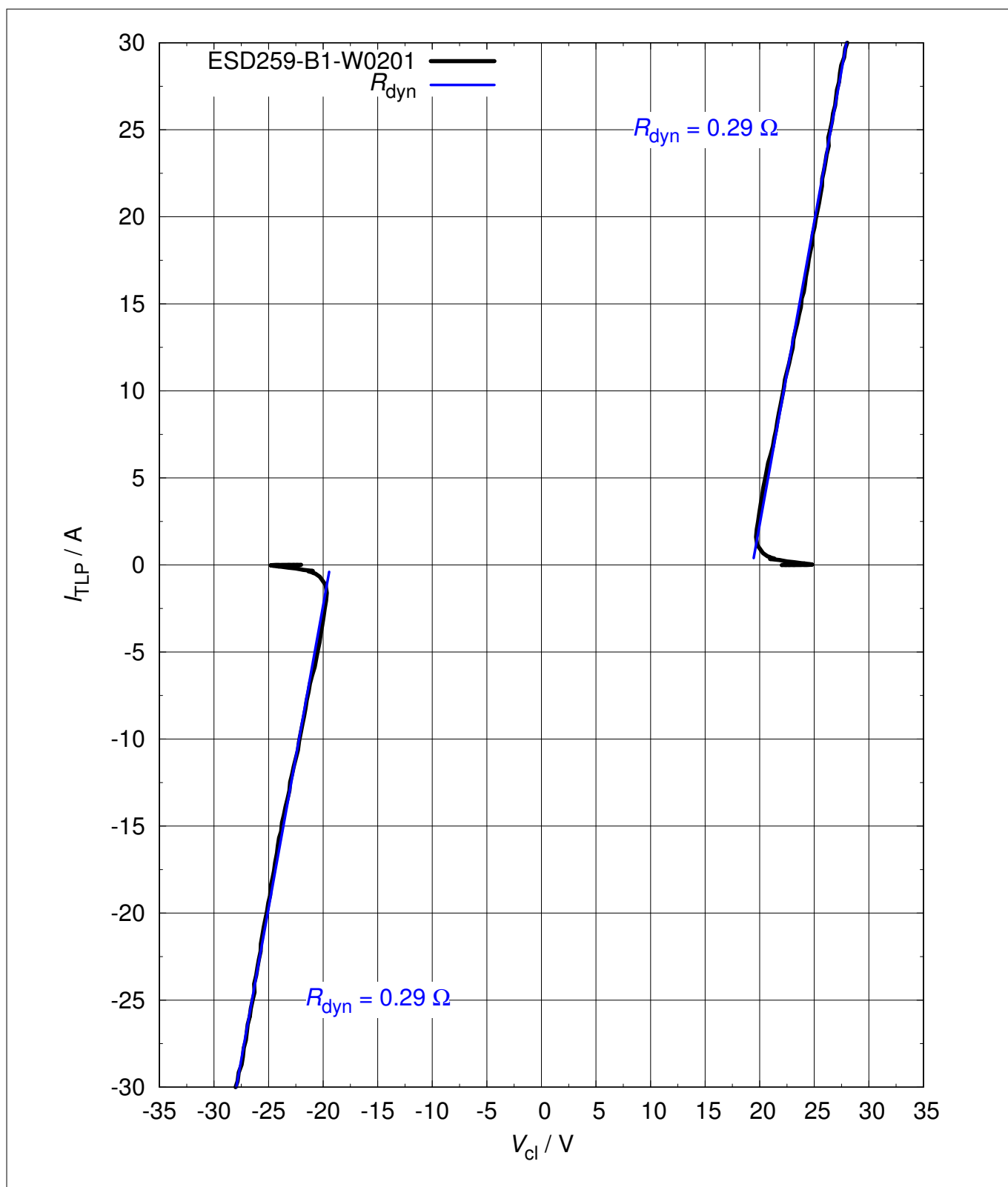
Figure 9 Clamping voltage (TLP): I_{TLP} = f(V_{cl})
