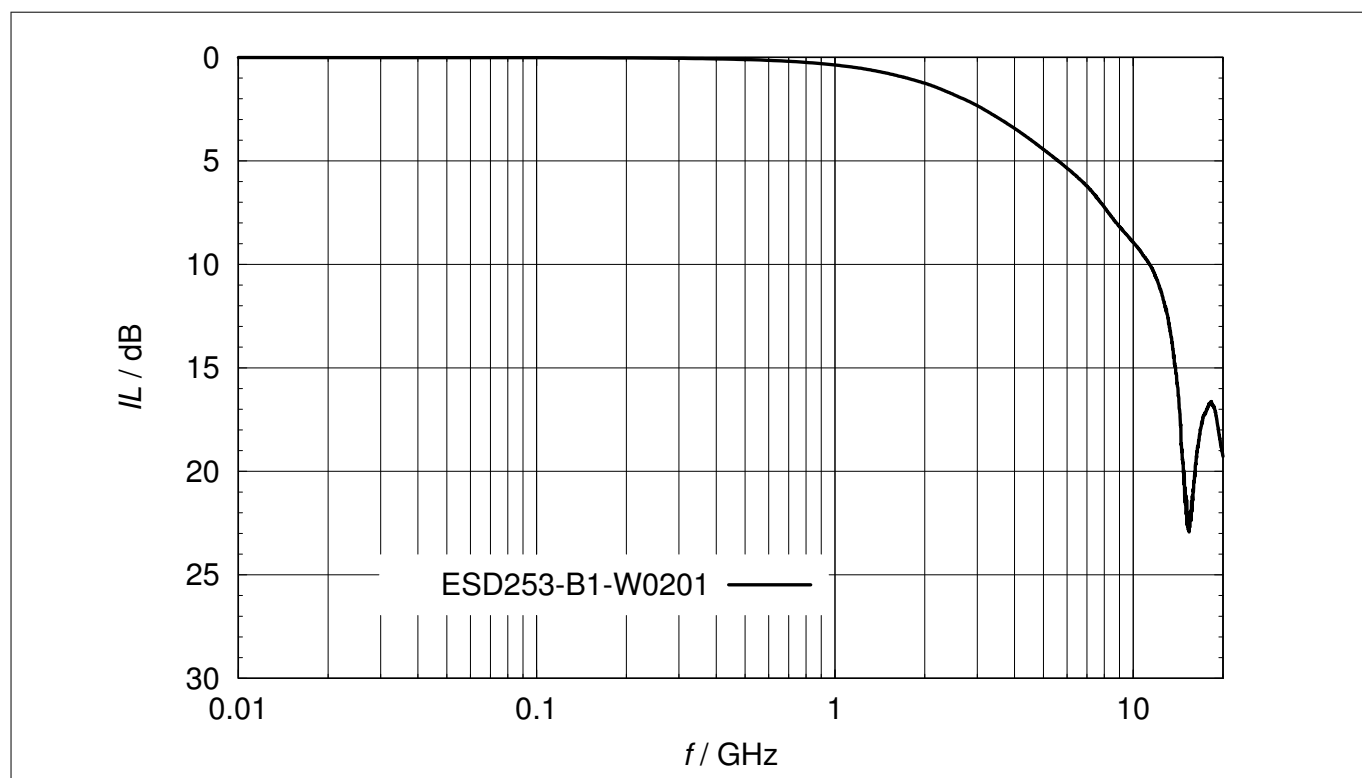
Figure 11 Insertion loss I_L = f(f) , in a 50 \Omega system
