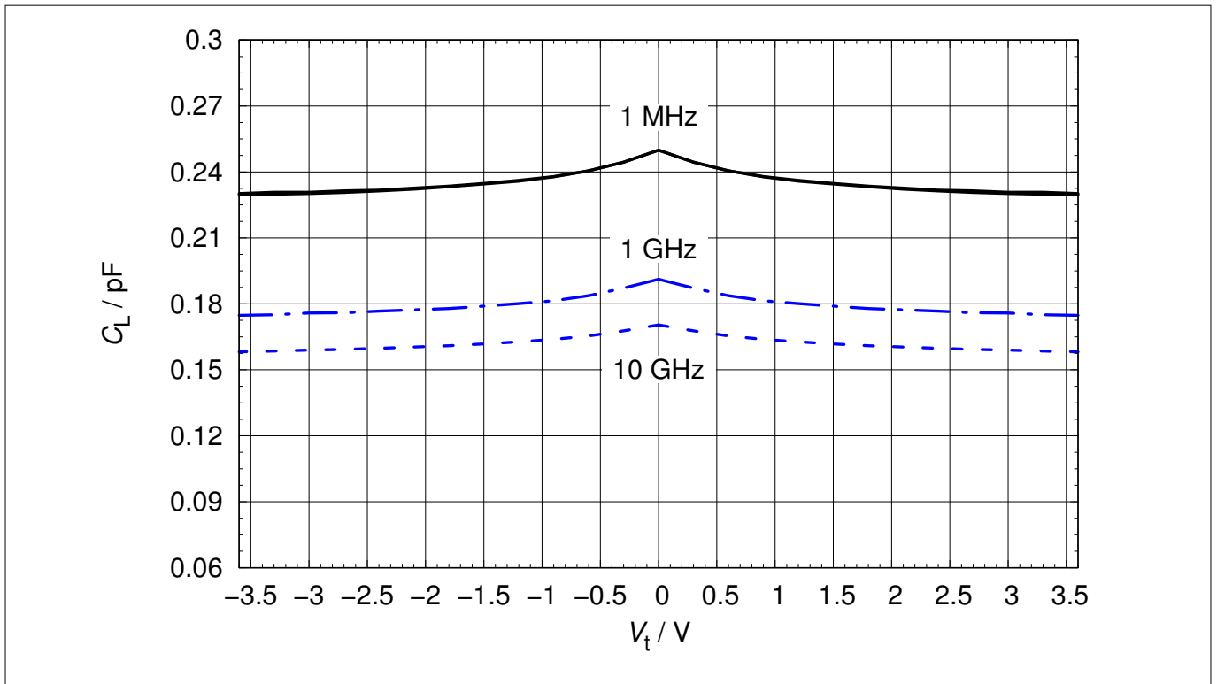
Figure 4 Line capacitance: C_L = f(V_t) , f = 1\text{ MHz}, 1\text{ GHz}, 10\text{ GHz}
