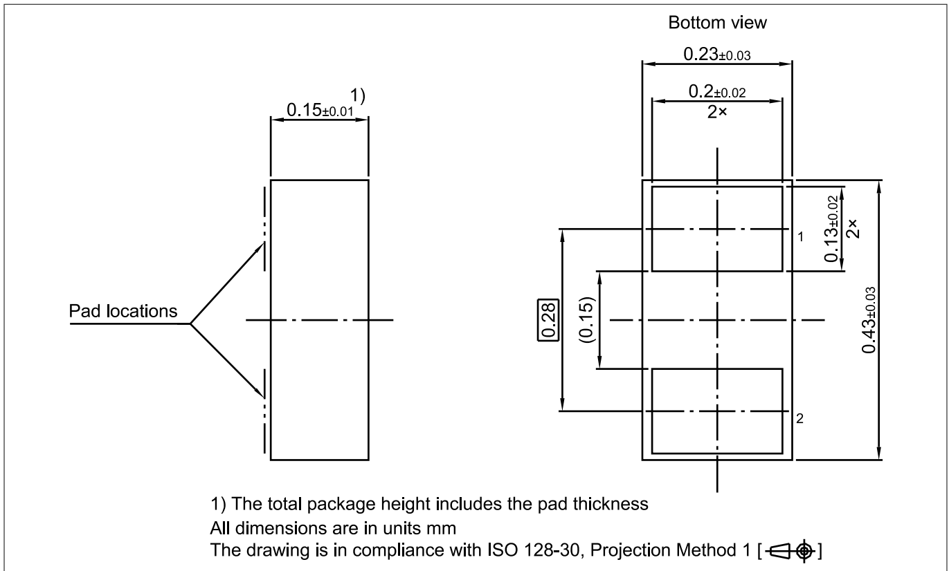
Figure 13 WLL-2-2 package
