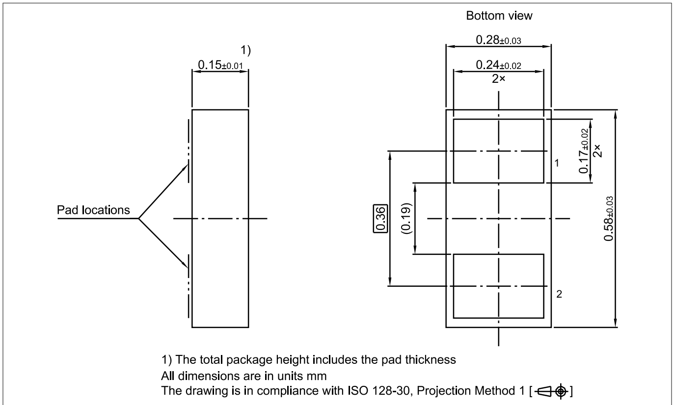
Figure 13 WLL-2-3 package
