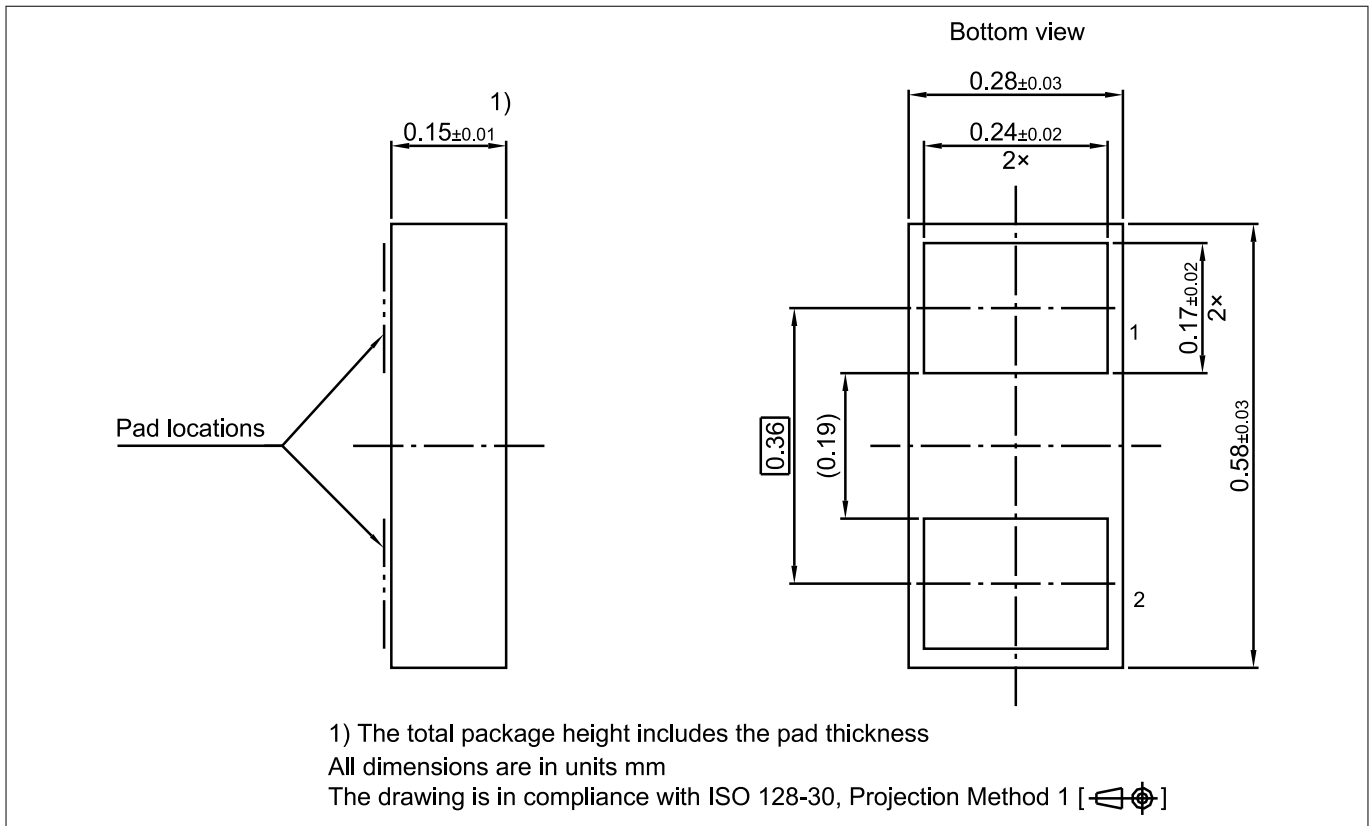
Figure 11 WLL-2-3 package
