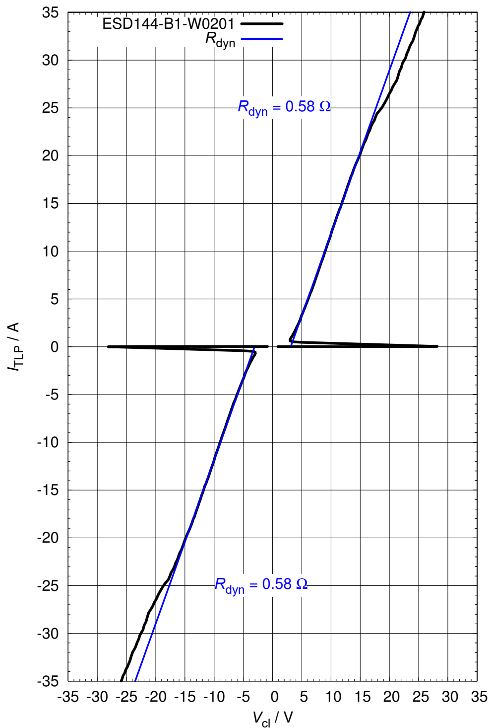
Figure 9 Clamping voltage (TLP): I_{TLP} = f(V_{cl})
