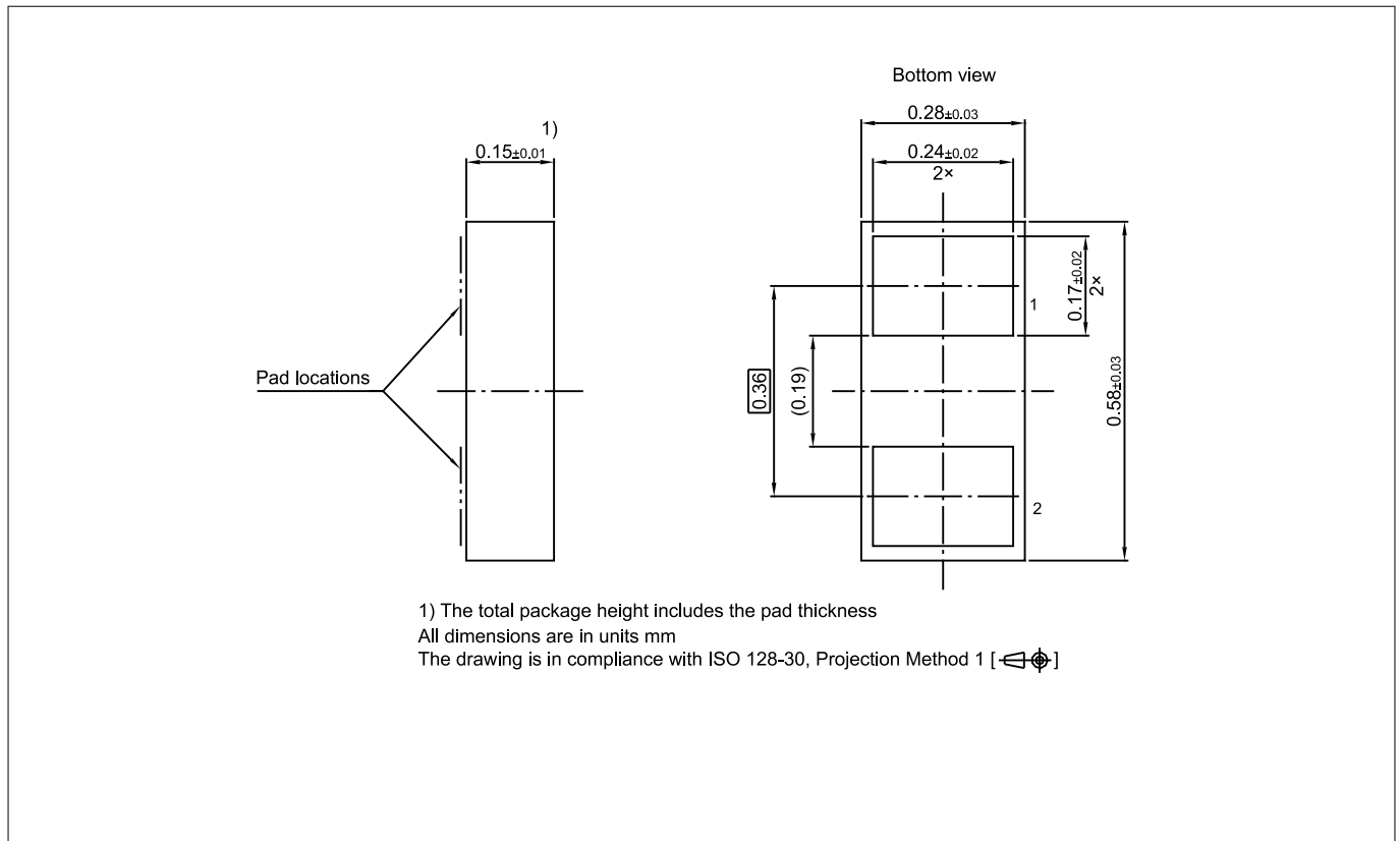
Figure 12 WLL-2-5 package
