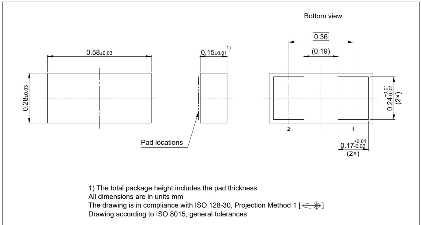
Figure 10 WLL-2-3 package
