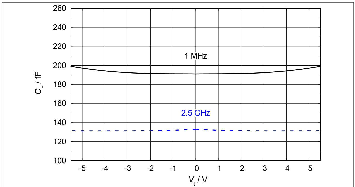
Figure 4 Line capacitance: C_L = f(V_t) , f = 1\text{ MHz}, 2.5\text{ GHz}
