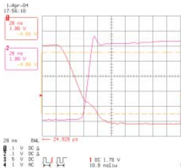
Figure 22. Turn-off Switching Waveform, Driving from a CD4049UB for Drain Current of 250mA
