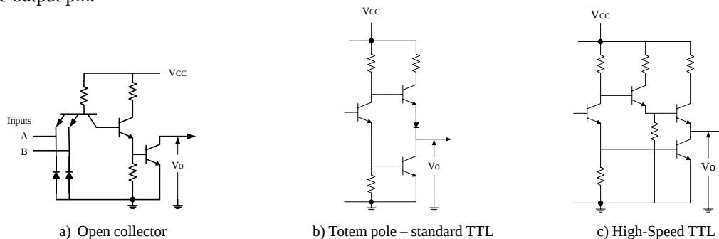
Figure 14. Simplified TTL Logic Gate Output Configurations
