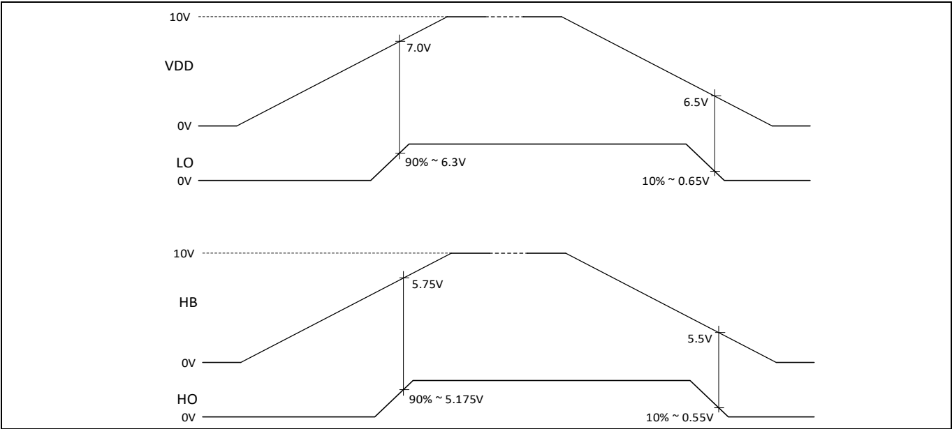
Figure 5 UVLO behavior
