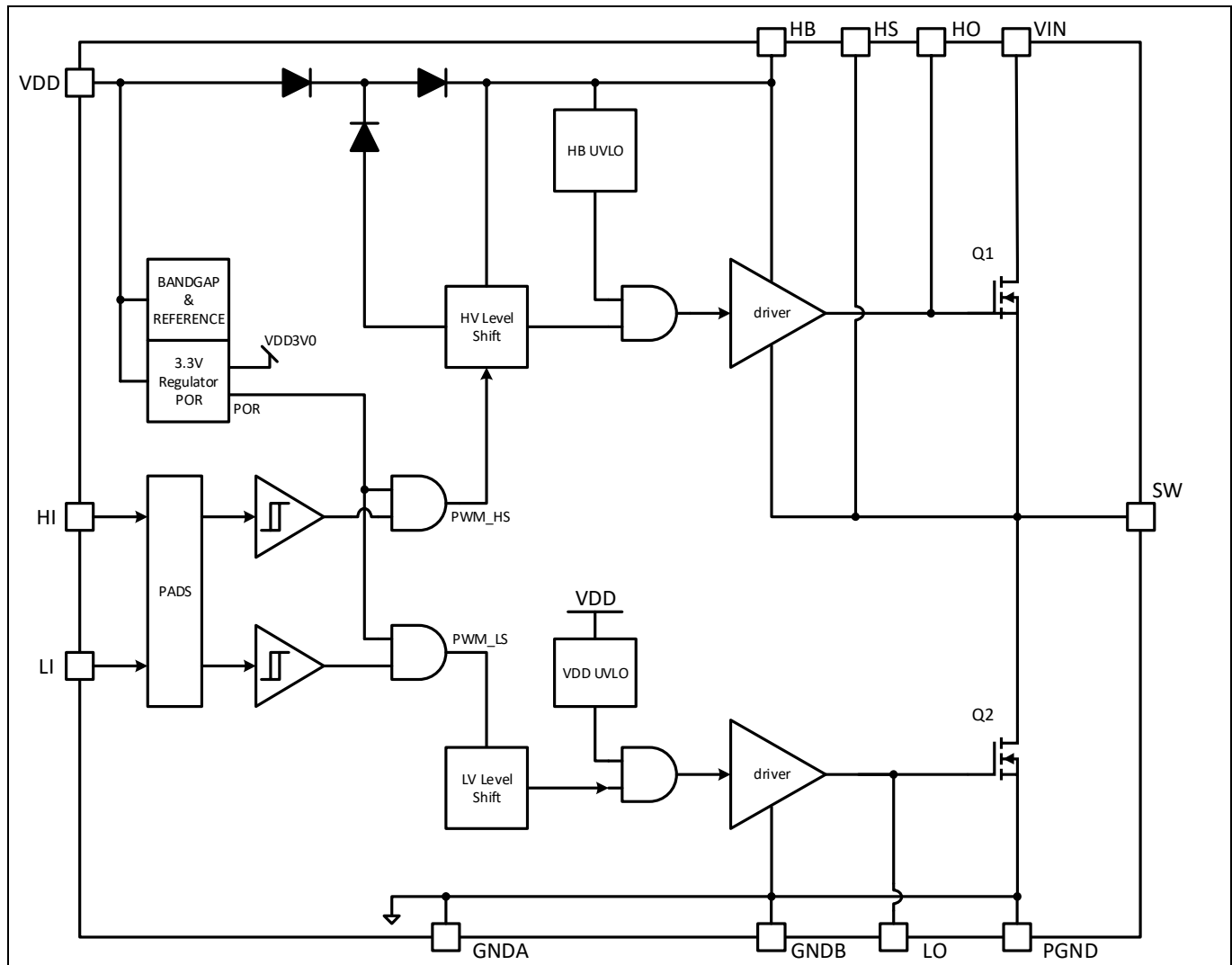
Figure 2 Block Diagram
