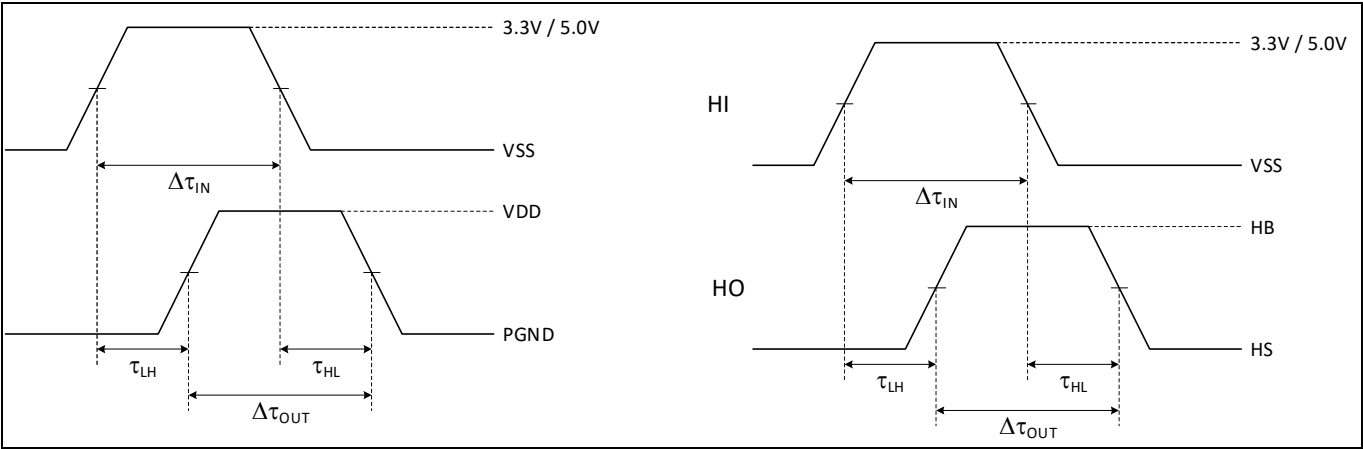
Figure 4 Propagation delay
