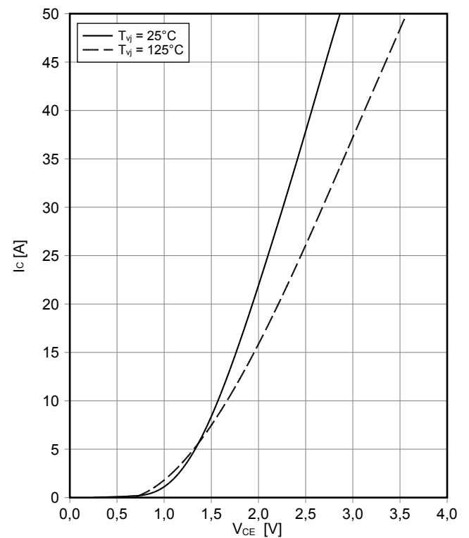
出力特性 IGBT、チョッパ ( Typical ) output characteristic IGBT-Chopper ( typical ) I_C = f(V_{CE}) V_{GE} = 15\text{ V}
